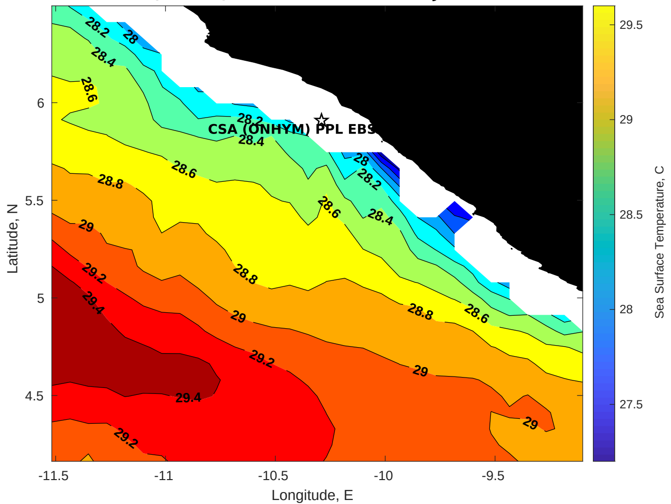
SST for CSA (ONHYM) PPL EBS - Liberia at 27-Jan-2026 00:00:00
