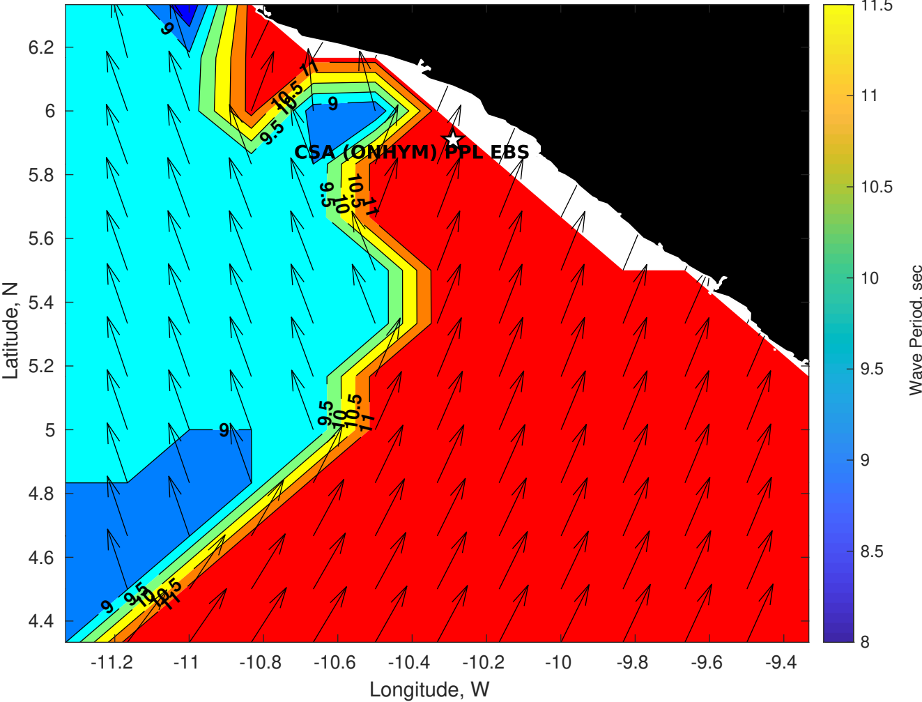
GFS Wave Period (sec) for CSA (ONHYM) PPL EBS - Liberia at 28-Jan-2026 09:00:00
