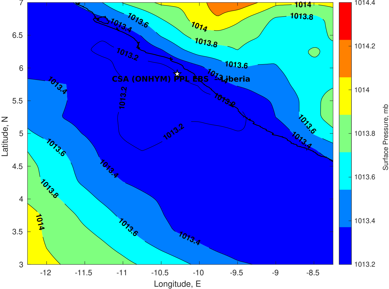
Surface Pressure (mb) for CSA (ONHYM) PPL EBS - Liberia at 29-Jan-2026 00:00:00
