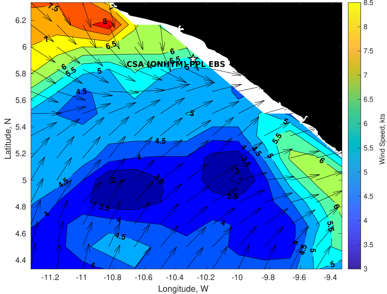
GFS Winds (kts) for CSA (ONHYM) PPL EBS - Liberia at 28-Jan-2026 09:00:00
