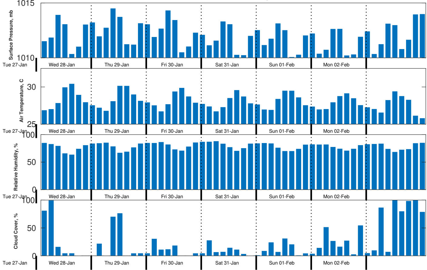
Met Forecast for CSA (ONHYM) PPL EBS - Liberia from 28-Jan-2026 00:00:00 to 04-Feb-2026 00:00:00
