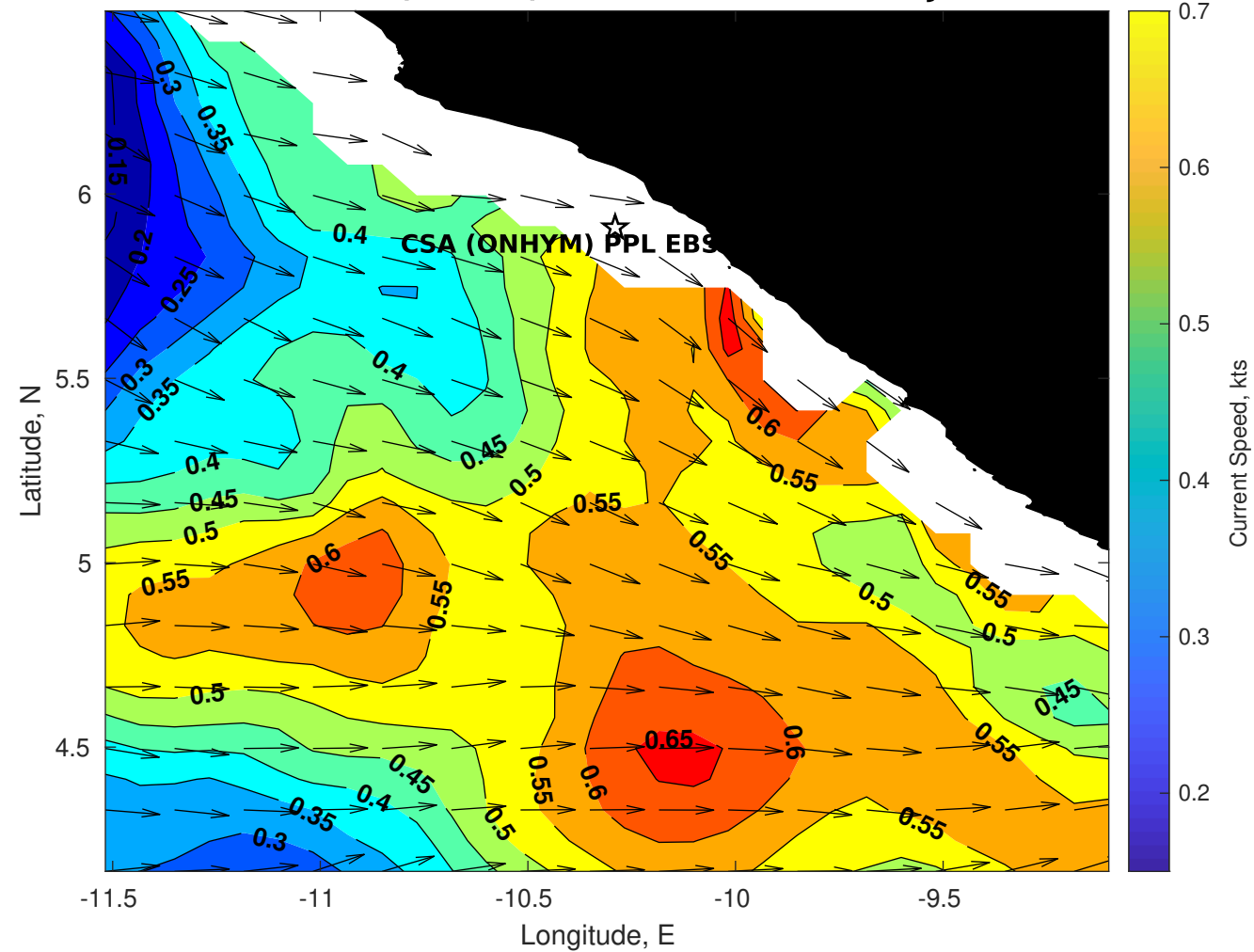
Surface Currents for CSA (ONHYM) PPL EBS - Liberia at 27-Jan-2026 00:00:00
