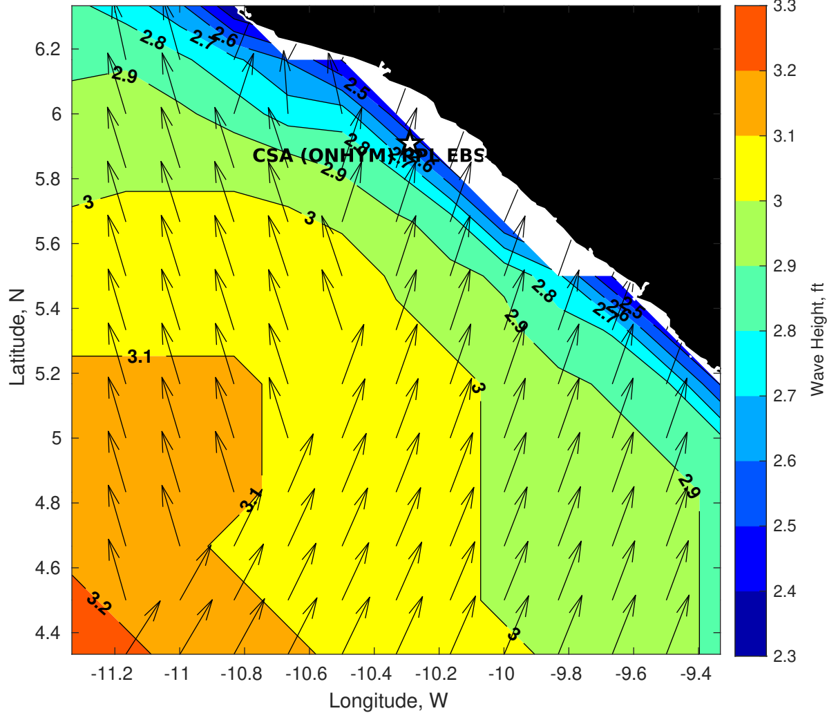
GFS Wave Height (ft) for CSA (ONHYM) PPL EBS - Liberia at 28-Jan-2026 09:00:00
