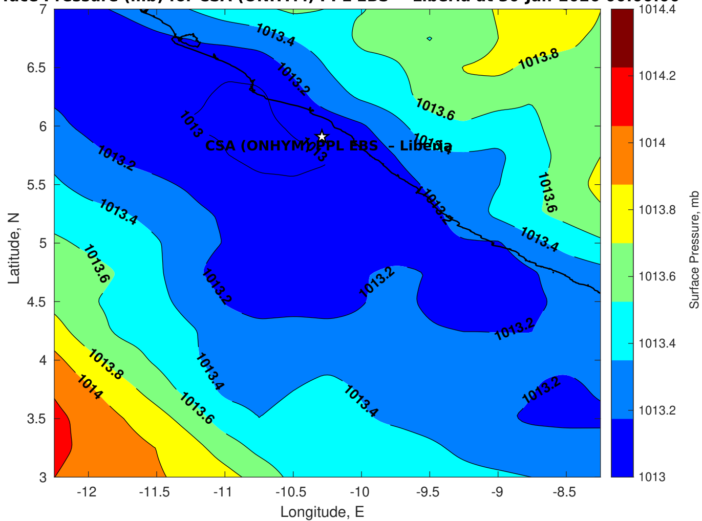
Surface Pressure (mb) for CSA (ONHYM) PPL EBS - Liberia at 30-Jan-2026 00:00:00
