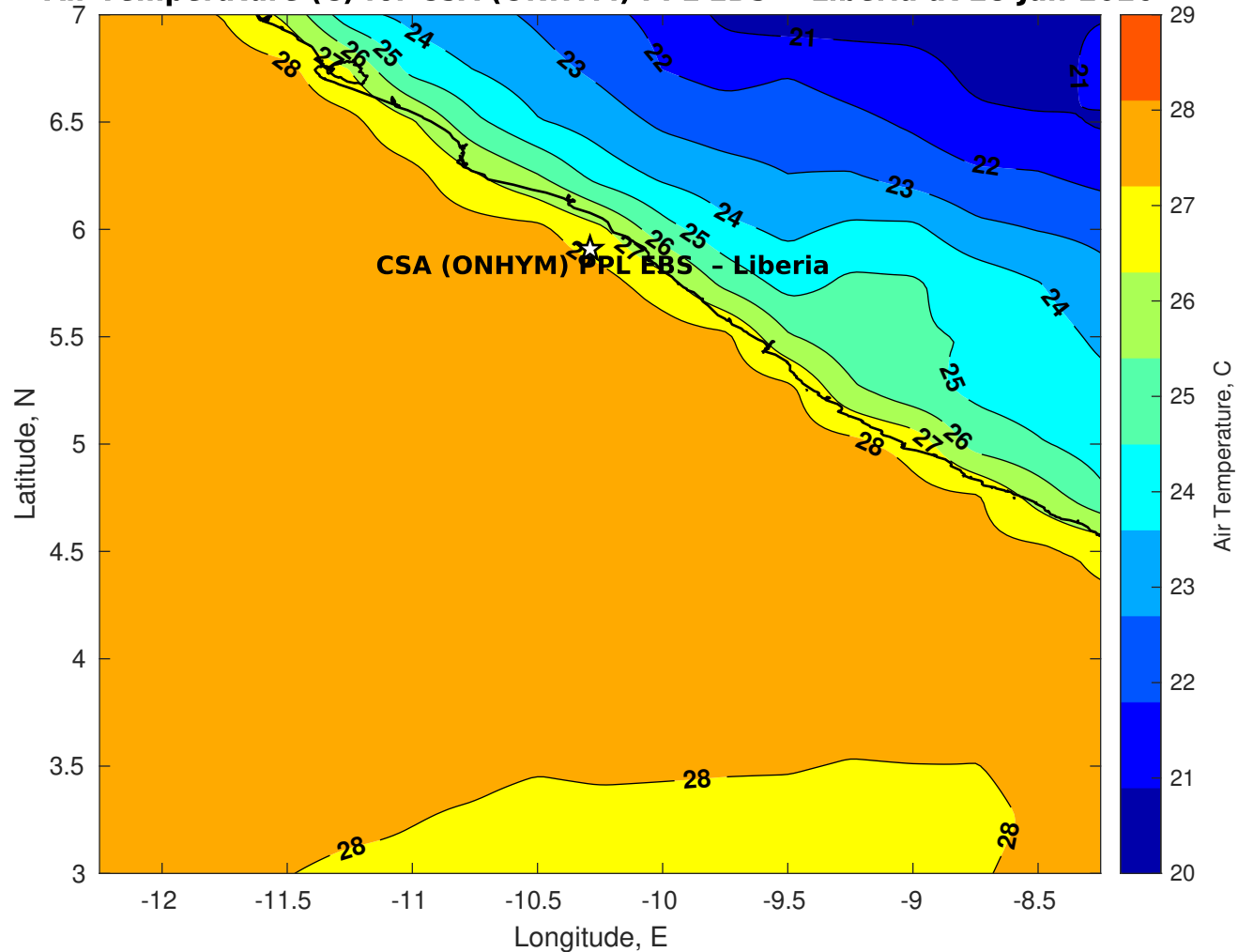
Air Temperature (C) for CSA (ONHYM) PPL EBS - Liberia at 28-Jan-2026
