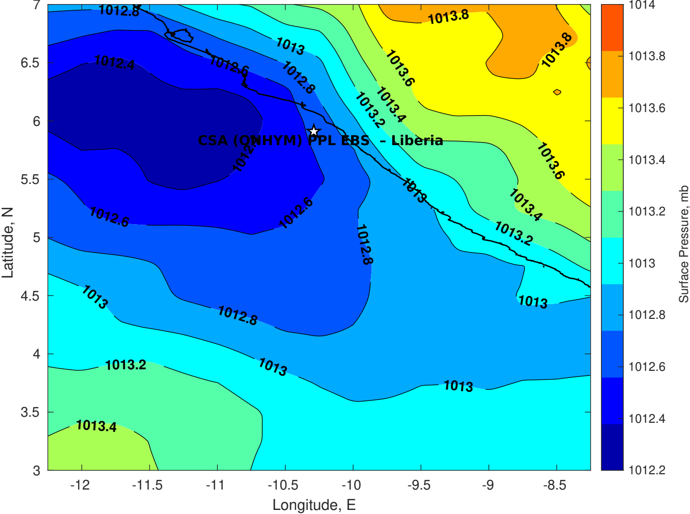
Surface Pressure (mb) for CSA (ONHYM) PPL EBS - Liberia at 28-Jan-2026 00:00:00
