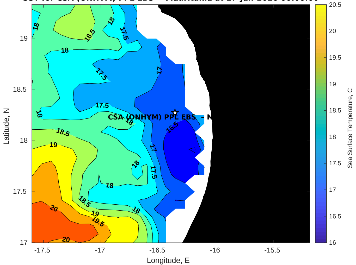
SST for CSA (ONHYM) PPL EBS - Mauritania at 27-Jan-2026 00:00:00
