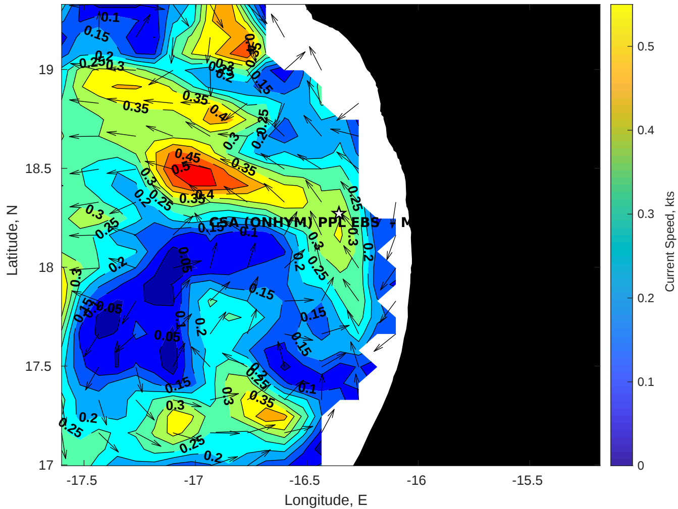
Surface Currents for CSA (ONHYM) PPL EBS - Mauritania at 27-Jan-2026 00:00:00
