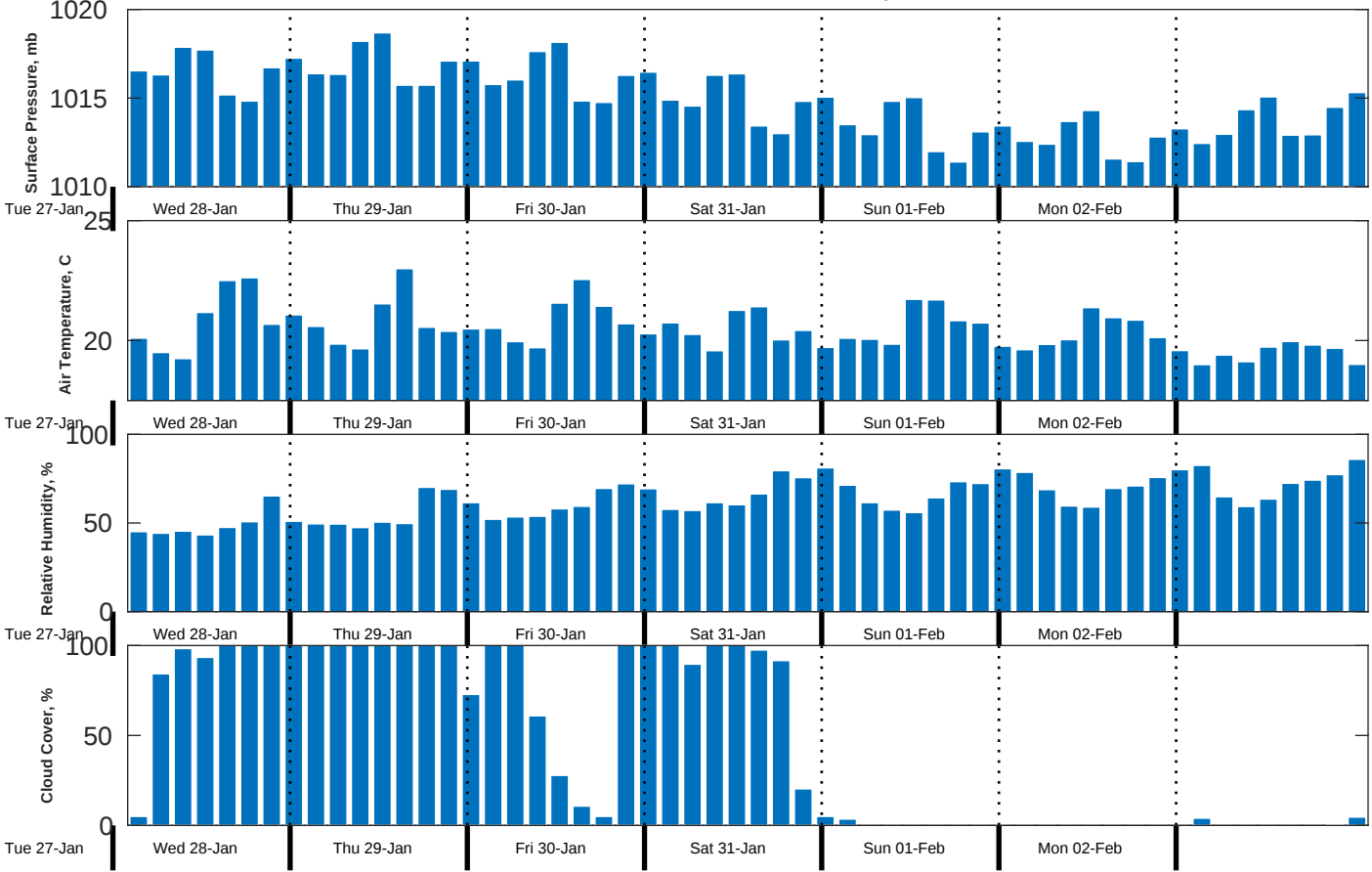
Met Forecast for CSA (ONHYM) PPL EBS - Mauritania from 28-Jan-2026 00:00:00 to 04-Feb-2026 00:00:00
