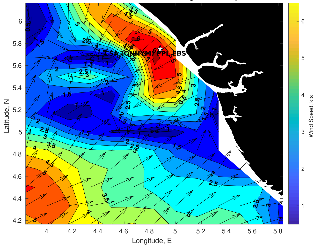
GFS Winds (kts) for CSA (ONHYM) PPL EBS - Nigeria at 28-Jan-2026 09:00:00
