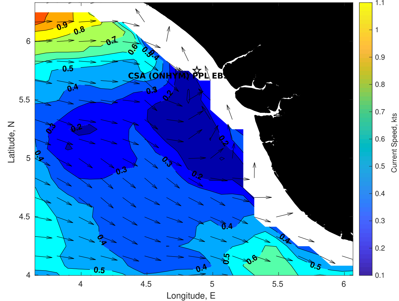
Surface Currents for CSA (ONHYM) PPL EBS - Nigeria at 27-Jan-2026 00:00:00
