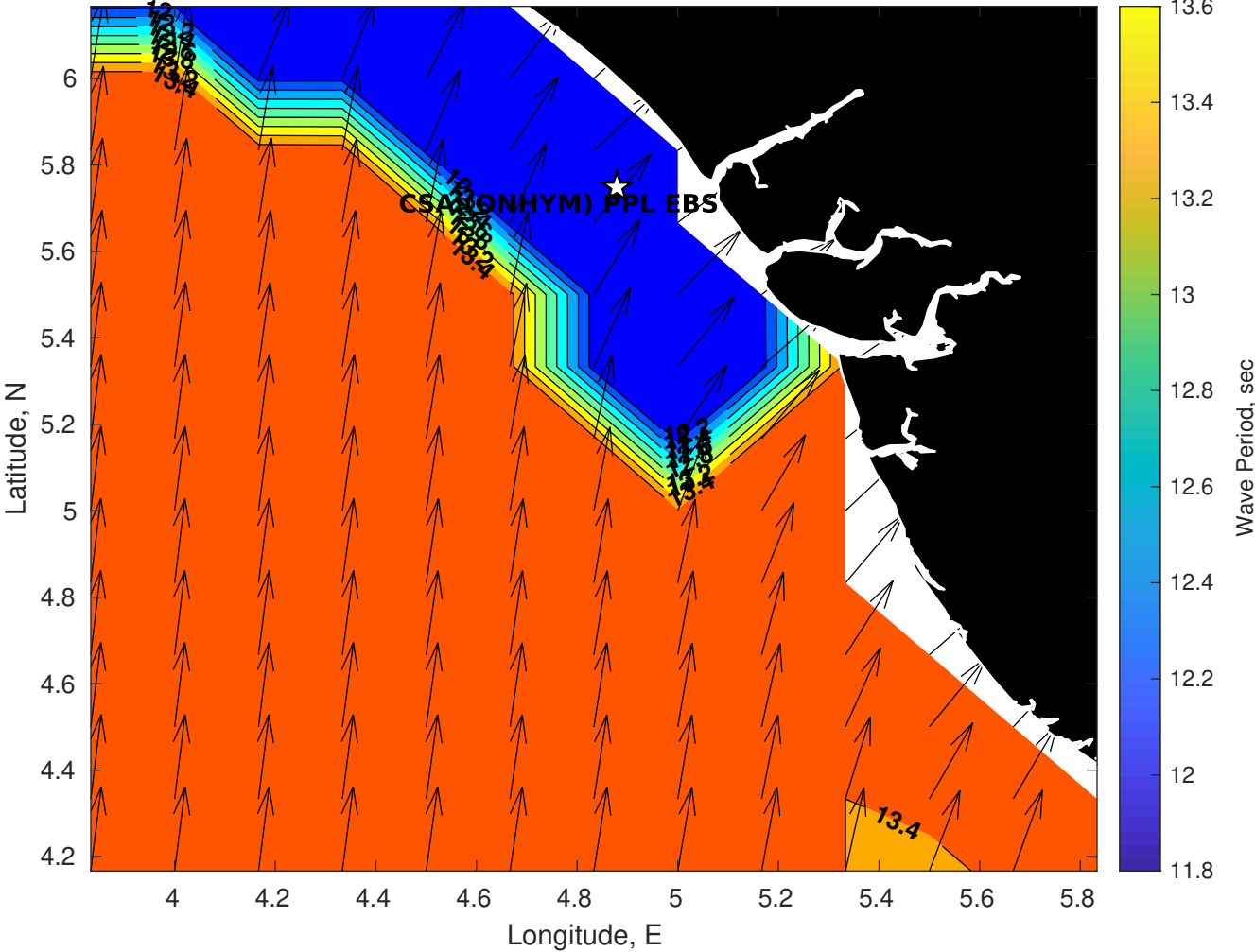
GFS Wave Period (sec) for CSA (ONHYM) PPL EBS - Nigeria at 28-Jan-2026 09:00:00
