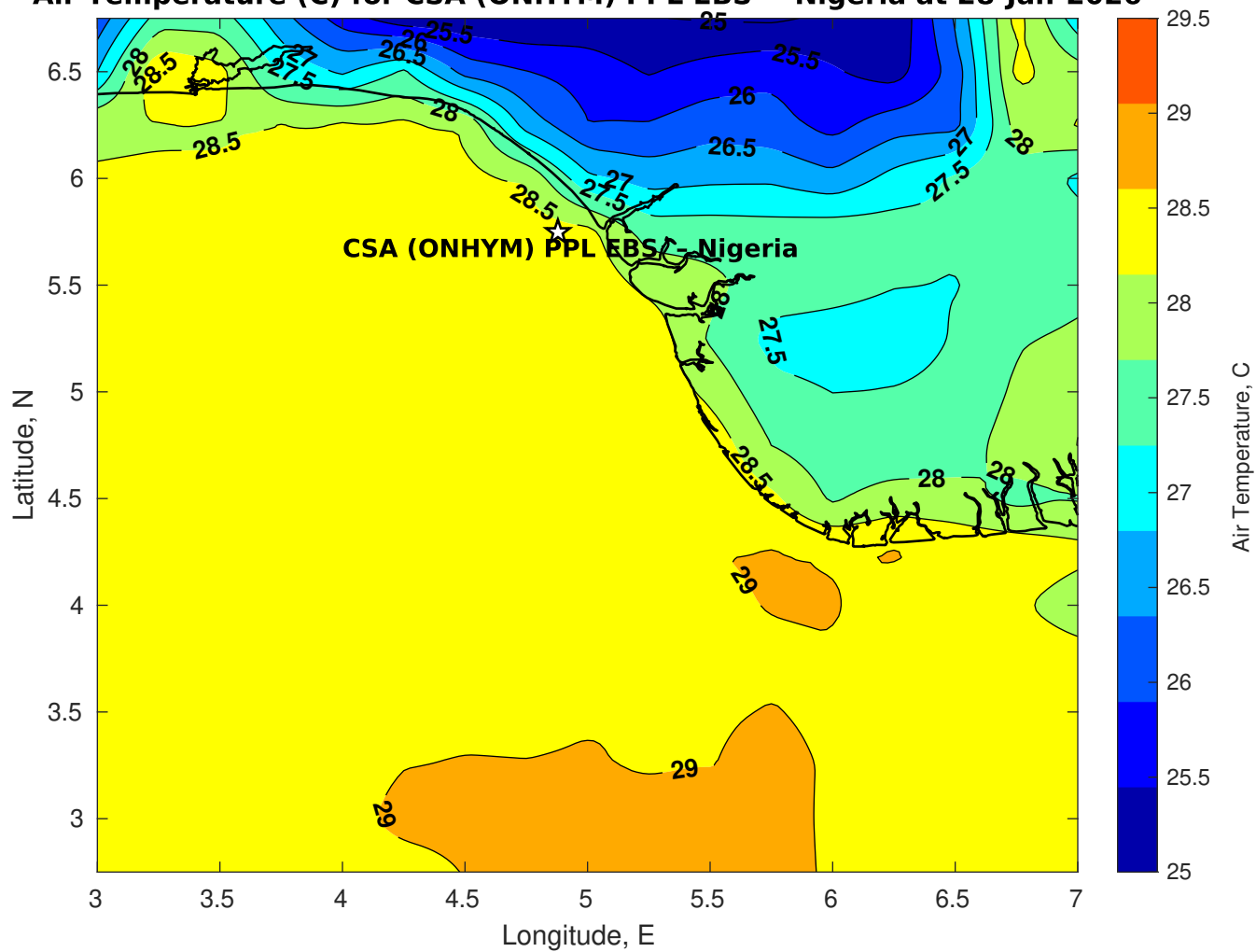
Air Temperature (C) for CSA (ONHYM) PPL EBS - Nigeria at 28-Jan-2026
