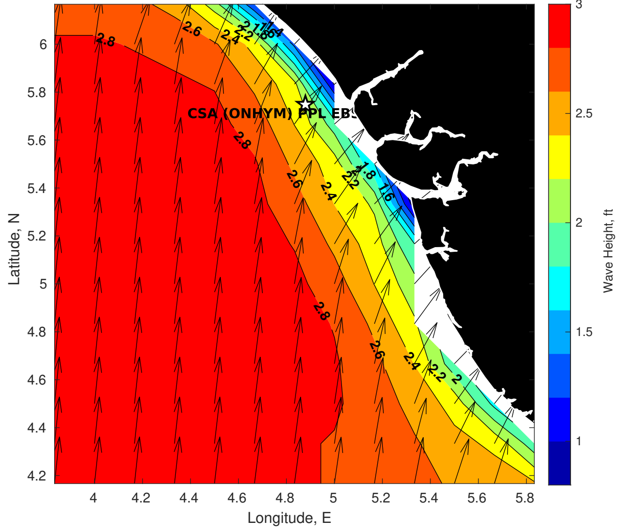
GFS Wave Height (ft) for CSA (ONHYM) PPL EBS - Nigeria at 28-Jan-2026 09:00:00
