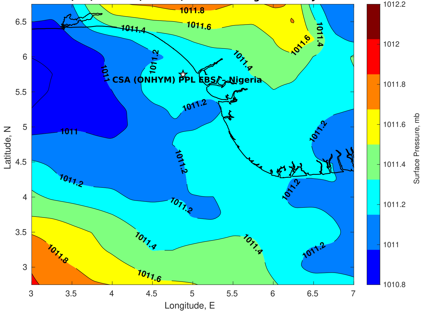
Surface Pressure (mb) for CSA (ONHYM) PPL EBS - Nigeria at 29-Jan-2026 00:00:00
