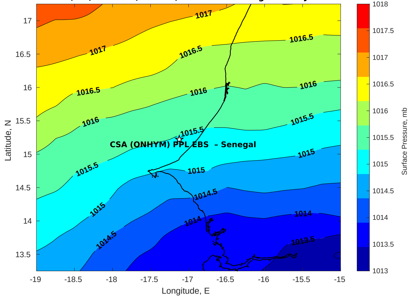
Surface Pressure (mb) for CSA (ONHYM) PPL EBS - Senegal at 28-Jan-2026 00:00:00
