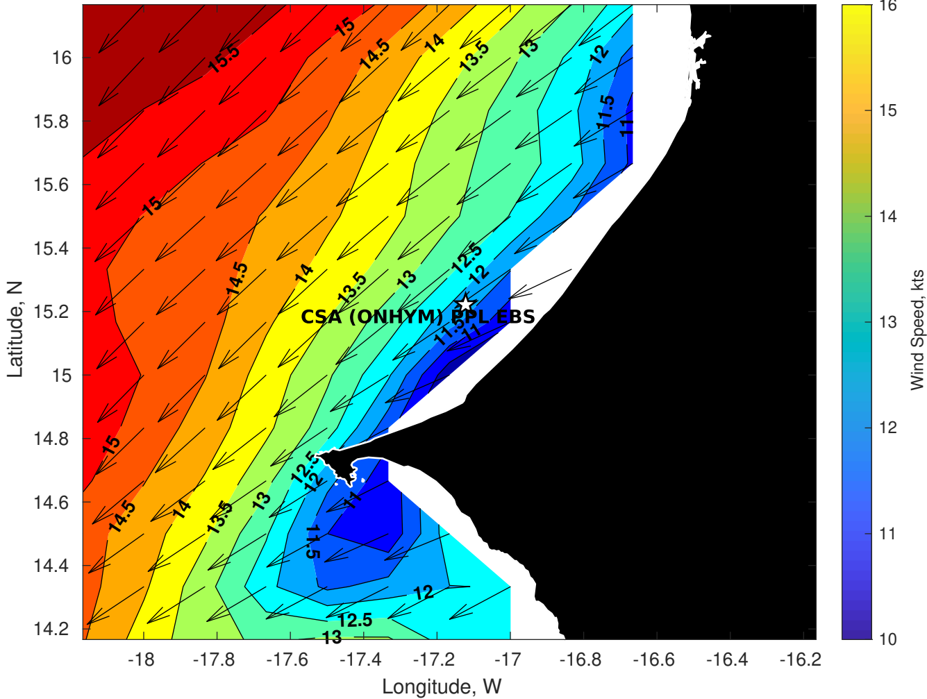
GFS Winds (kts) for CSA (ONHYM) PPL EBS - Senegal at 28-Jan-2026 09:00:00
