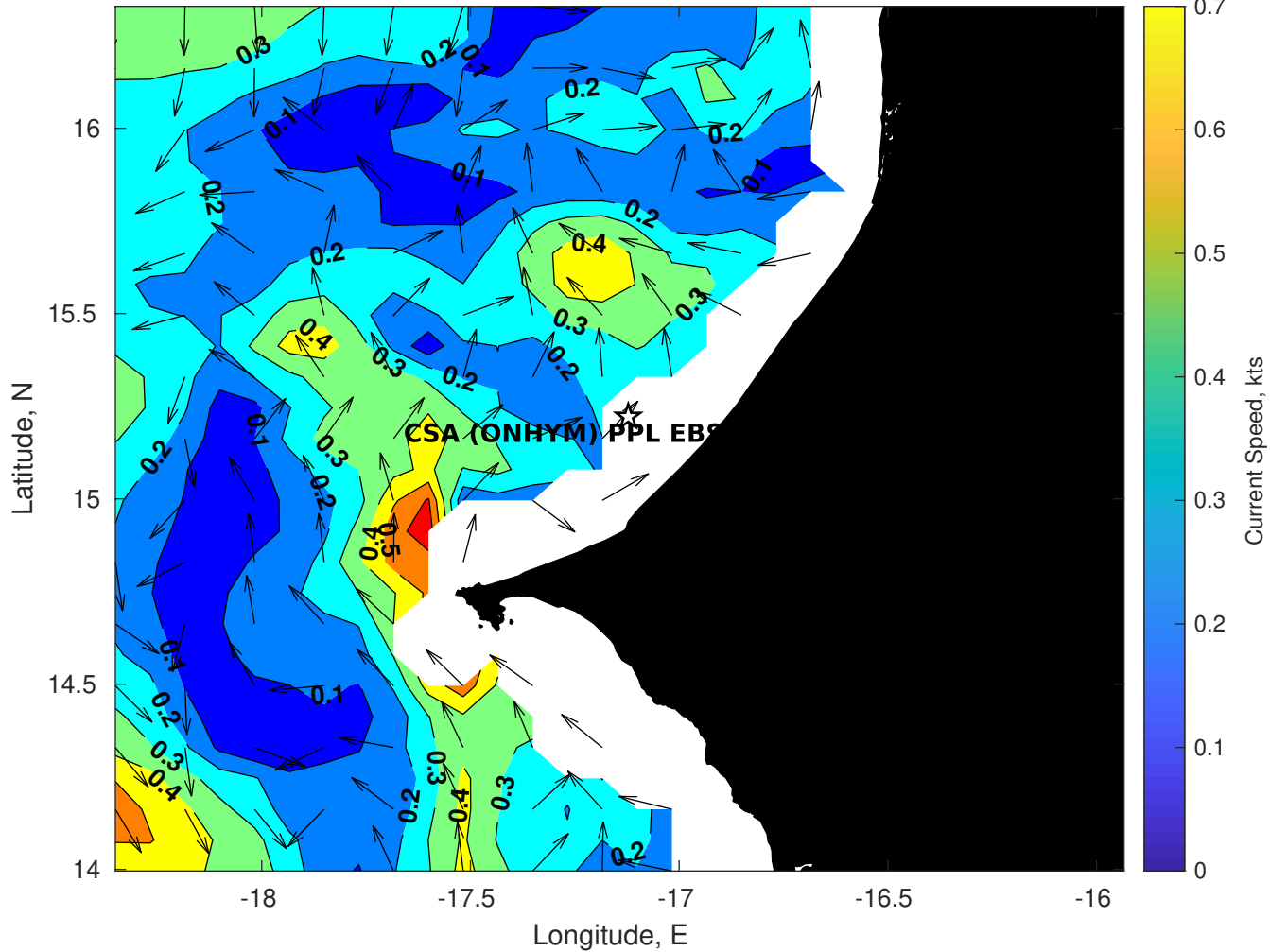
Surface Currents for CSA (ONHYM) PPL EBS - Senegal at 27-Jan-2026 00:00:00
