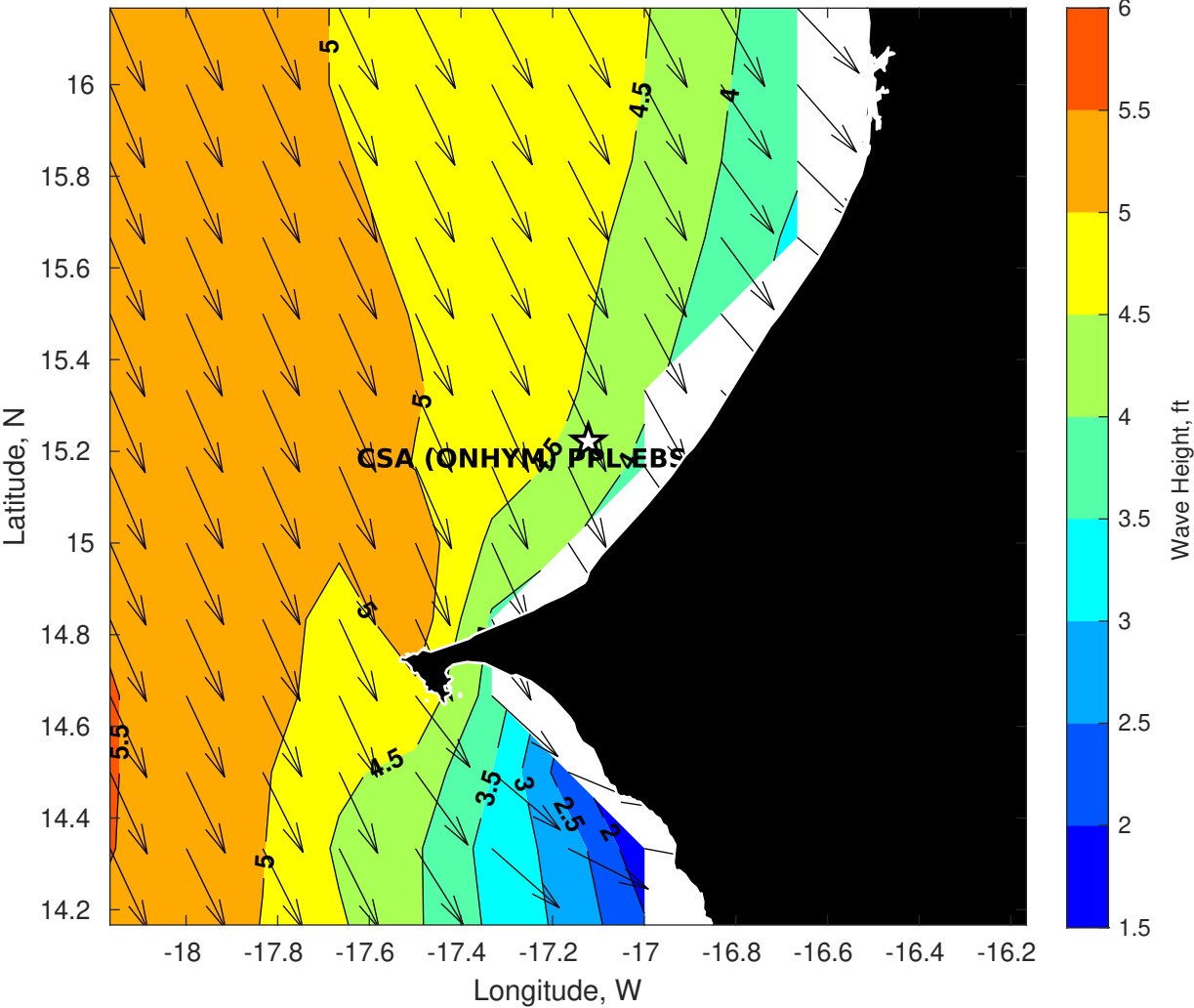
GFS Wave Height (ft) for CSA (ONHYM) PPL EBS - Senegal at 28-Jan-2026 09:00:00
