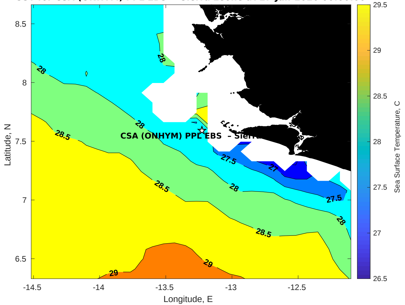
SST for CSA (ONHYM) PPL EBS - Sierra Leone at 27-Jan-2026 00:00:00
