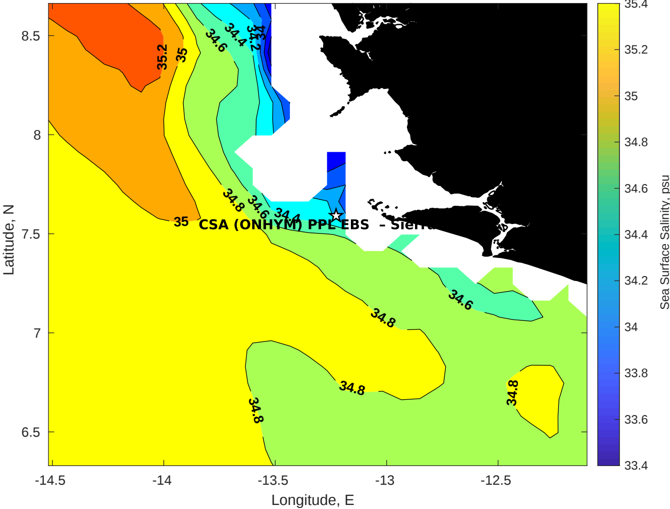
Surface Salinity for CSA (ONHYM) PPL EBS - Sierra Leone at 27-Jan-2026 00:00:00
