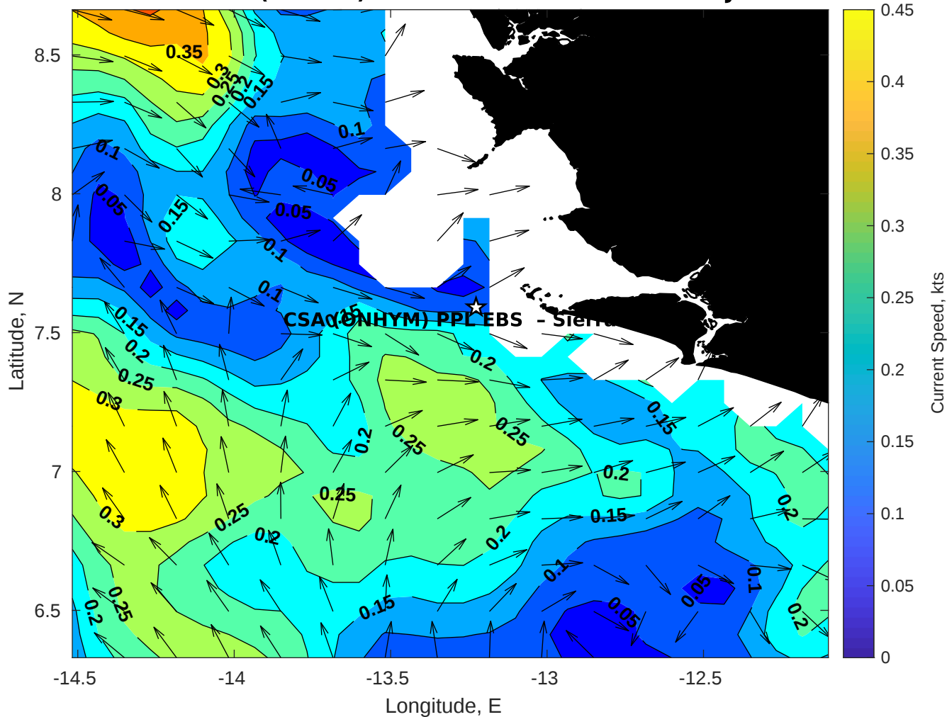
Surface Currents for CSA (ONHYM) PPL EBS - Sierra Leone at 27-Jan-2026 00:00:00
