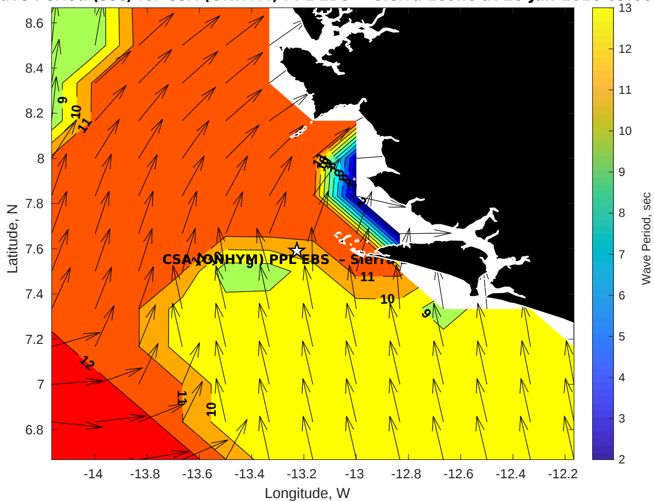
GFS Wave Period (sec) for CSA (ONHYM) PPL EBS - Sierra Leone at 28-Jan-2026 09:00:00
