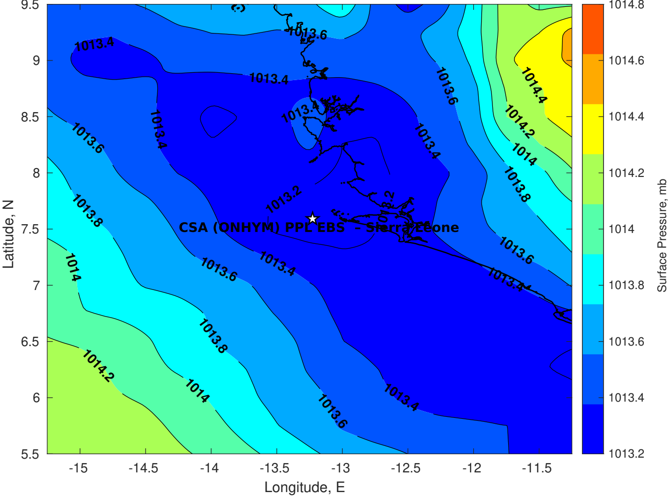
Surface Pressure (mb) for CSA (ONHYM) PPL EBS - Sierra Leone at 29-Jan-2026 00:00:00
