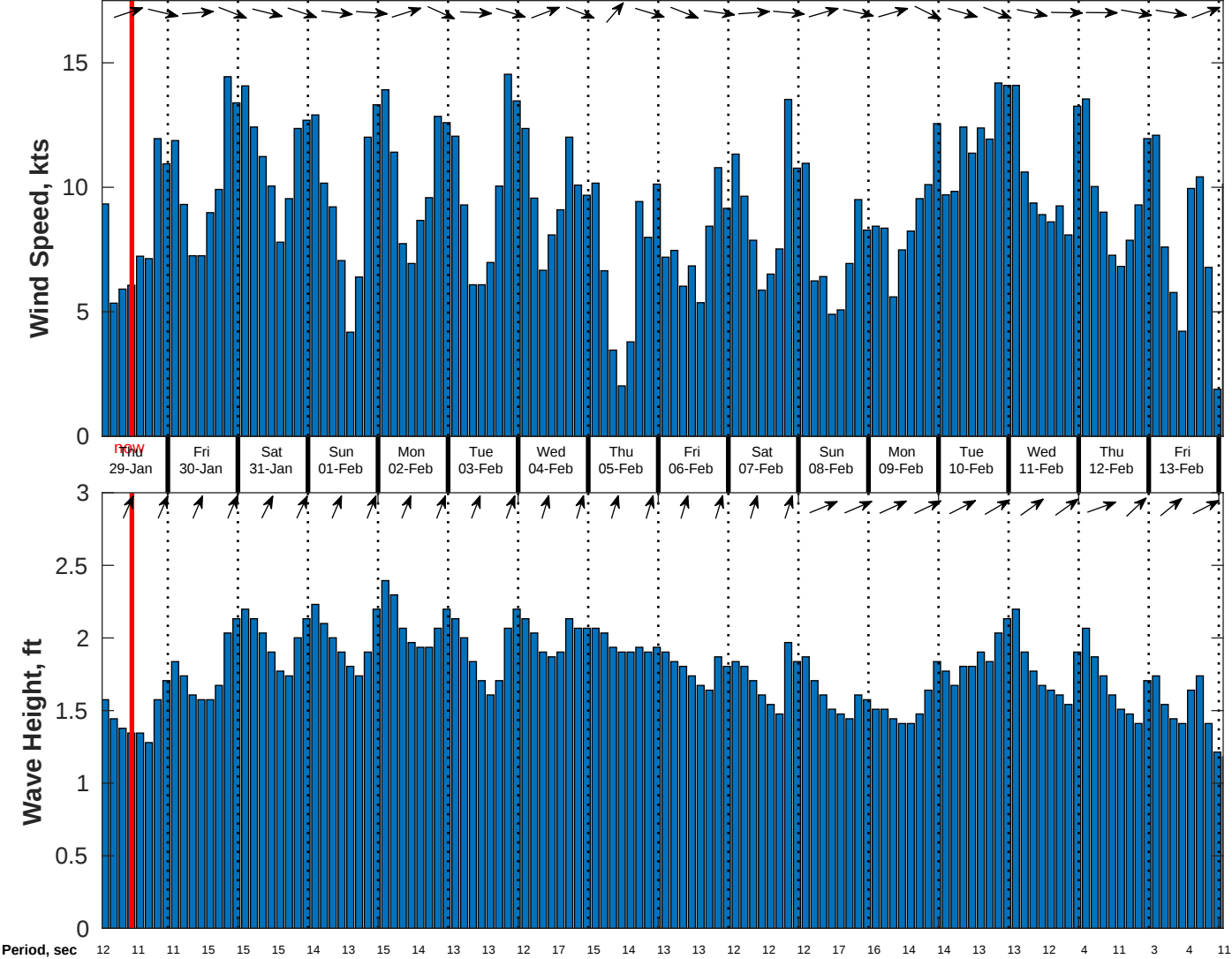
Wind & Wave Forecast for CSA (ONHYM) PPL EBS - Sierra Leone from 28-Jan-2026 01:00:00 to 13-Feb-2026 01:00:00
