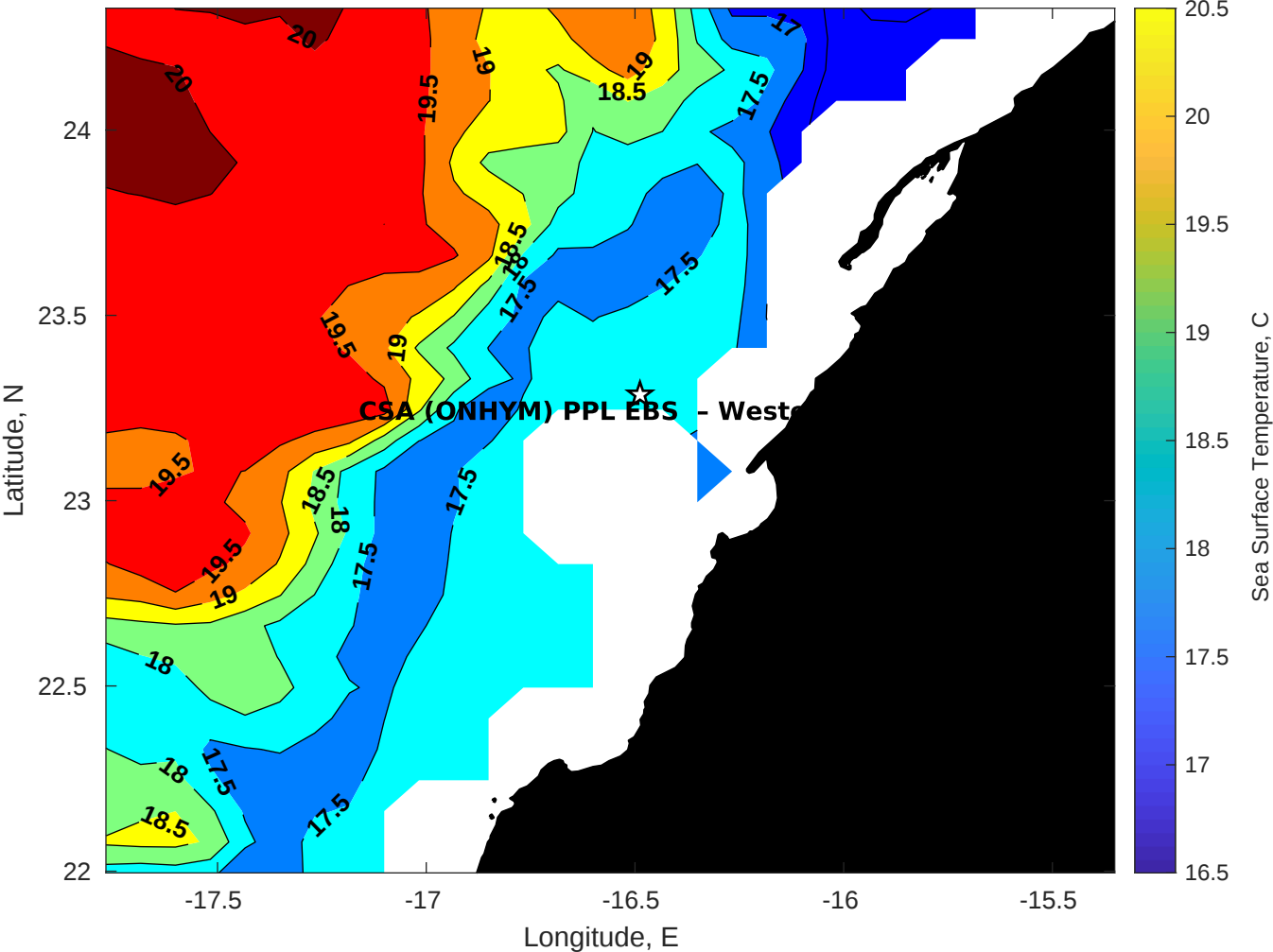
SST for CSA (ONHYM) PPL EBS - Western Sahara at 27-Jan-2026 00:00:00
