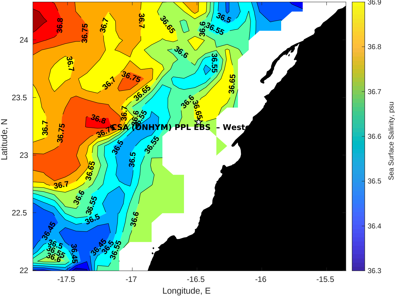
Surface Salinity for CSA (ONHYM) PPL EBS - Western Sahara at 27-Jan-2026 00:00:00
