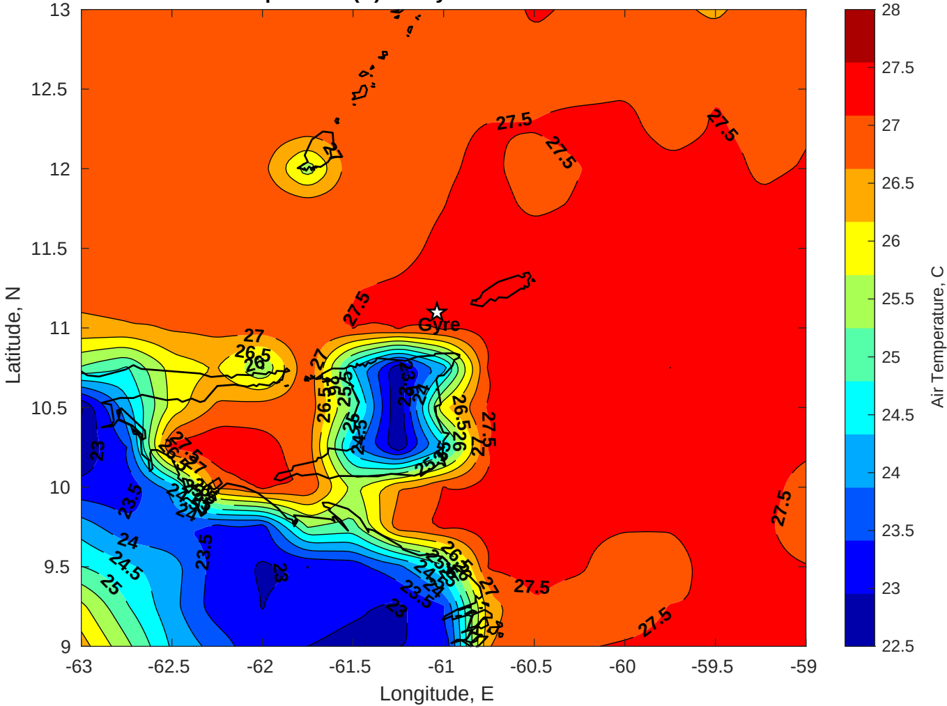
Air Temperature (C) for Gyre at 28-Jan-2026
