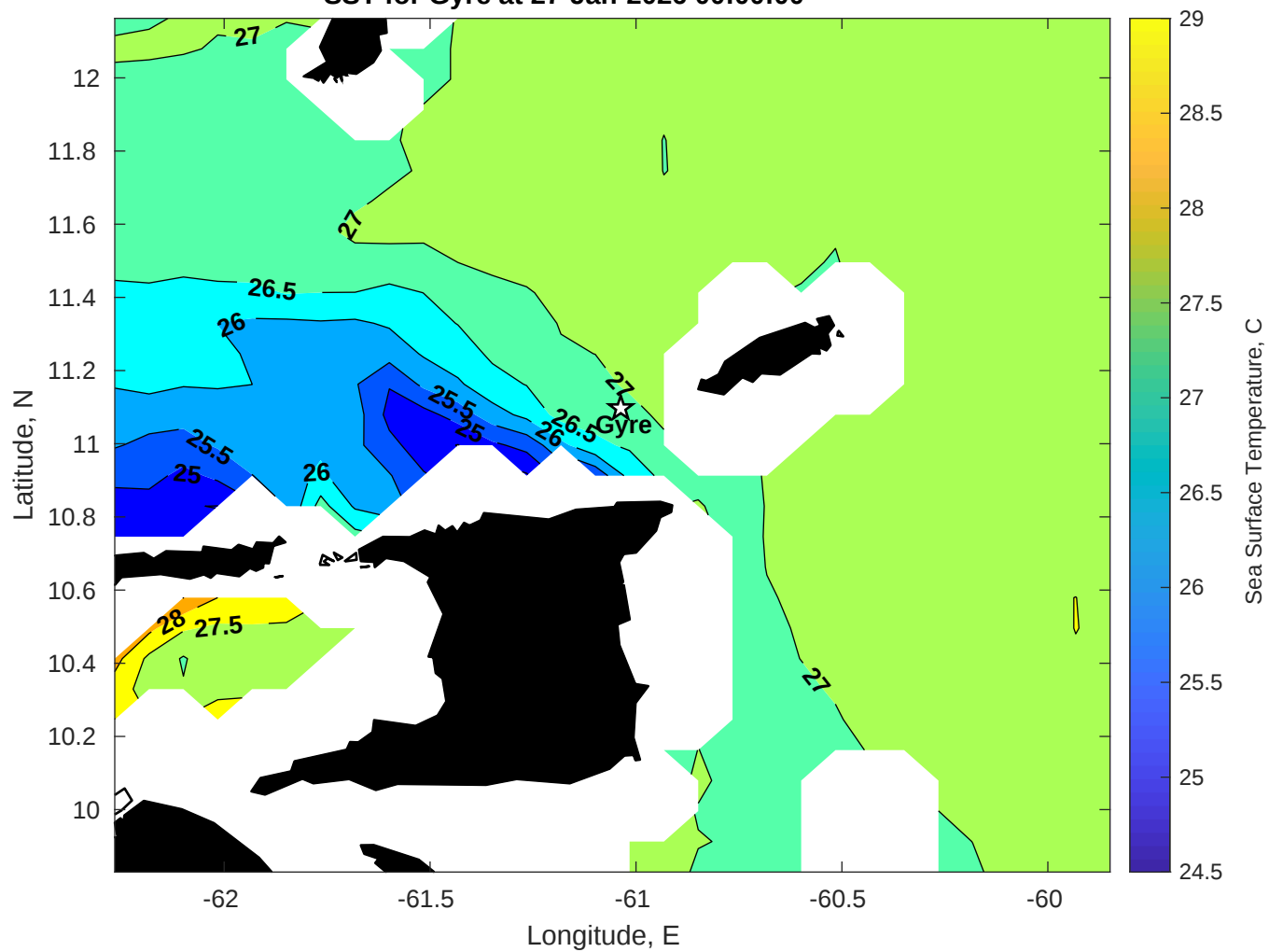
SST for Gyre at 27-Jan-2026 00:00:00
