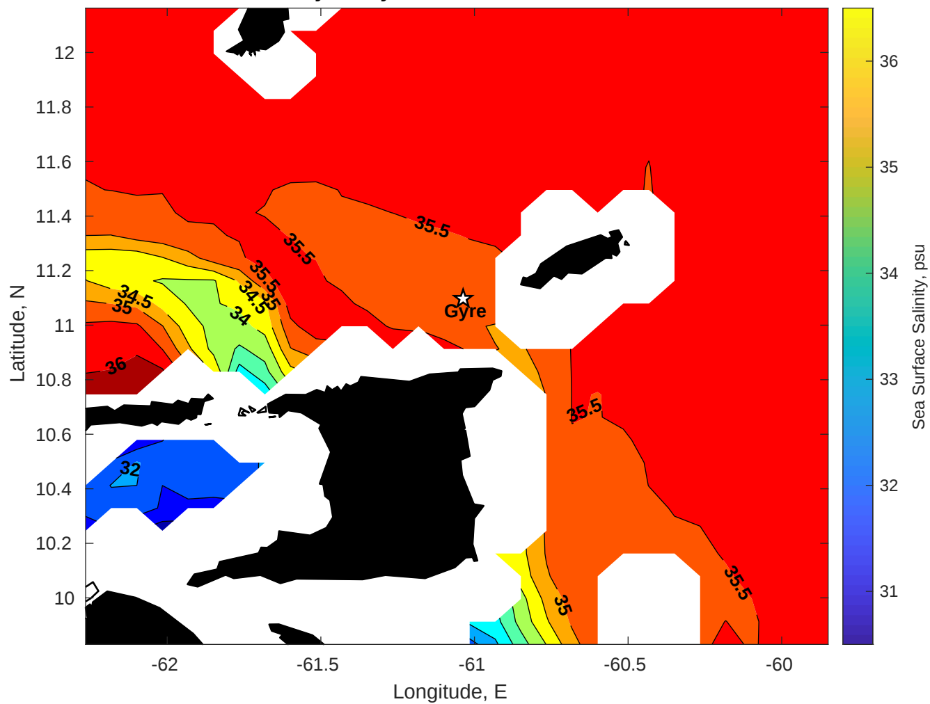
Surface Salinity for Gyre at 27-Jan-2026 00:00:00
