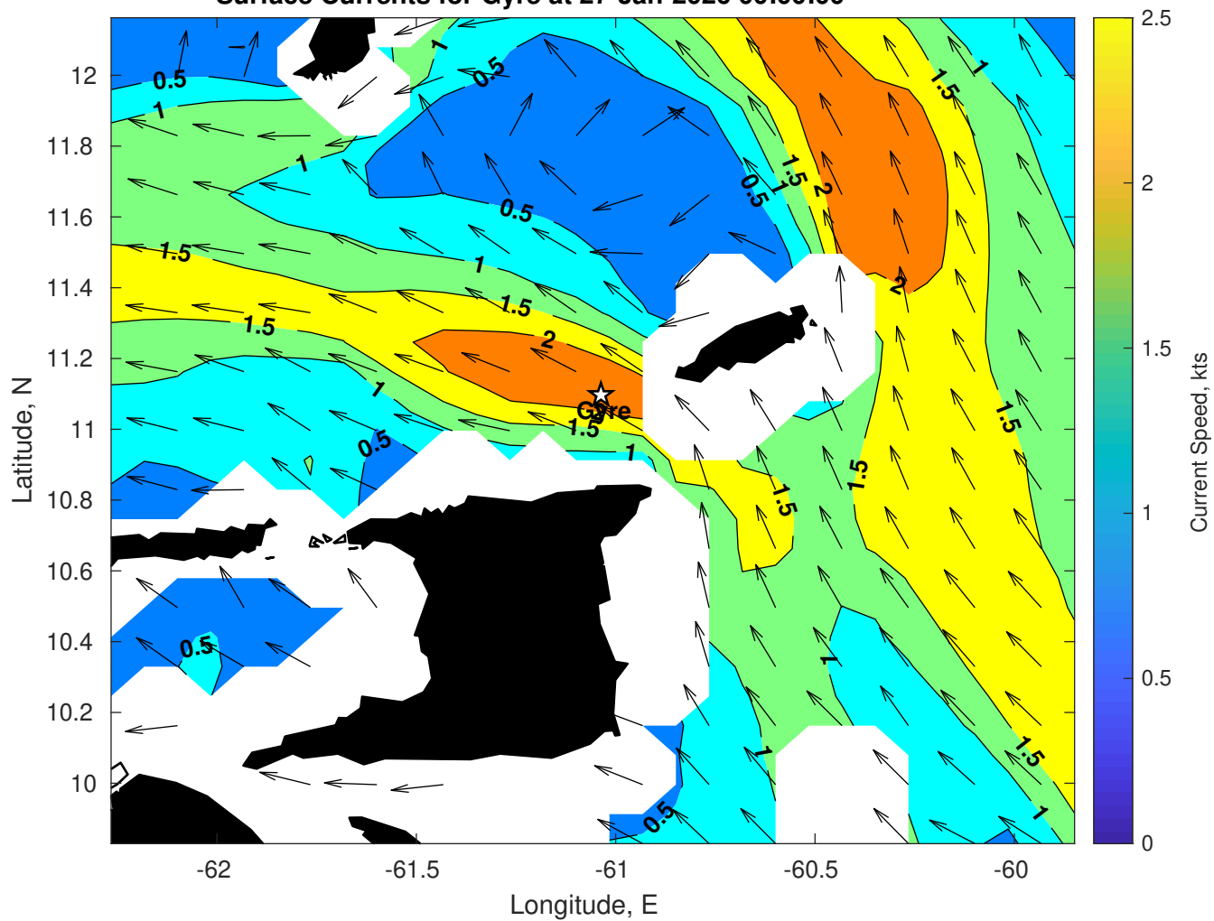
Surface Currents for Gyre at 27-Jan-2026 00:00:00
