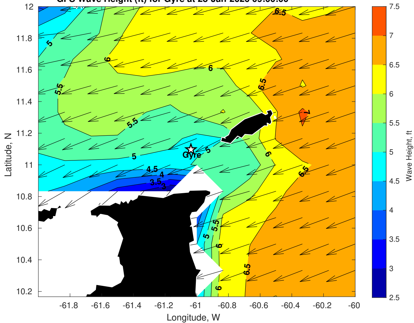
GFS Wave Height (ft) for Gyre at 28-Jan-2026 09:00:00
