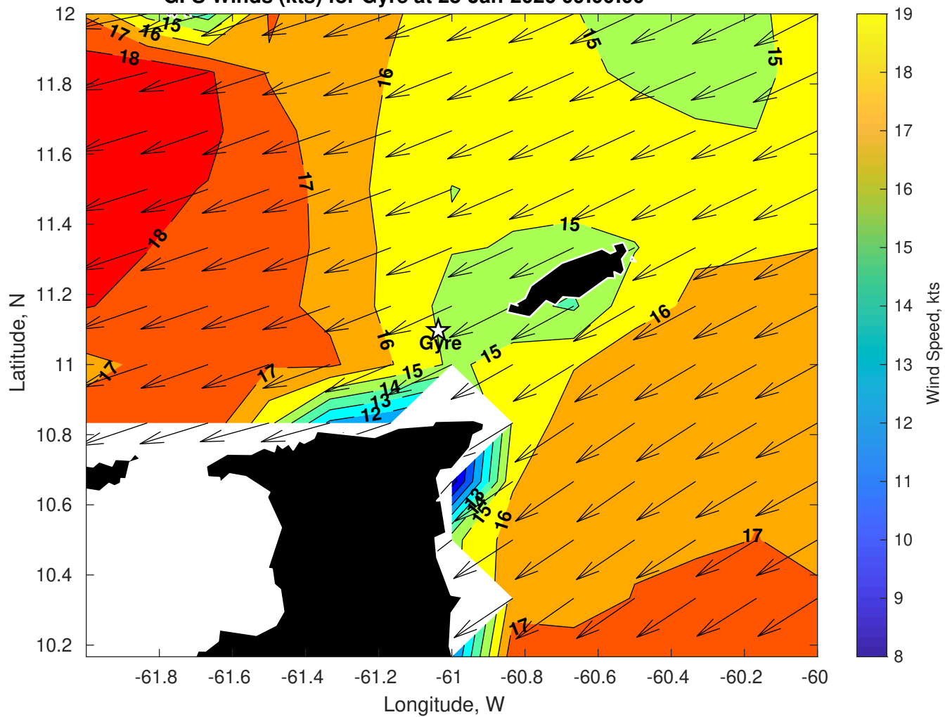
GFS Winds (kts) for Gyre at 28-Jan-2026 09:00:00
