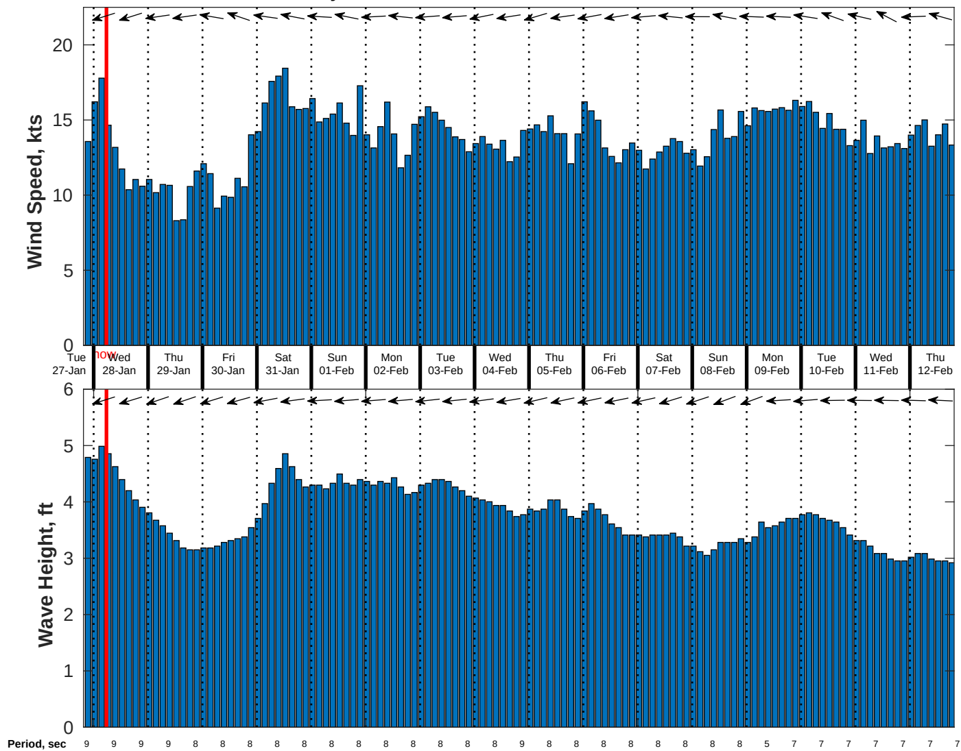
Wind & Wave Forecast for Gyre from 27-Jan-2026 20:00:00 to 12-Feb-2026 20:00:00
