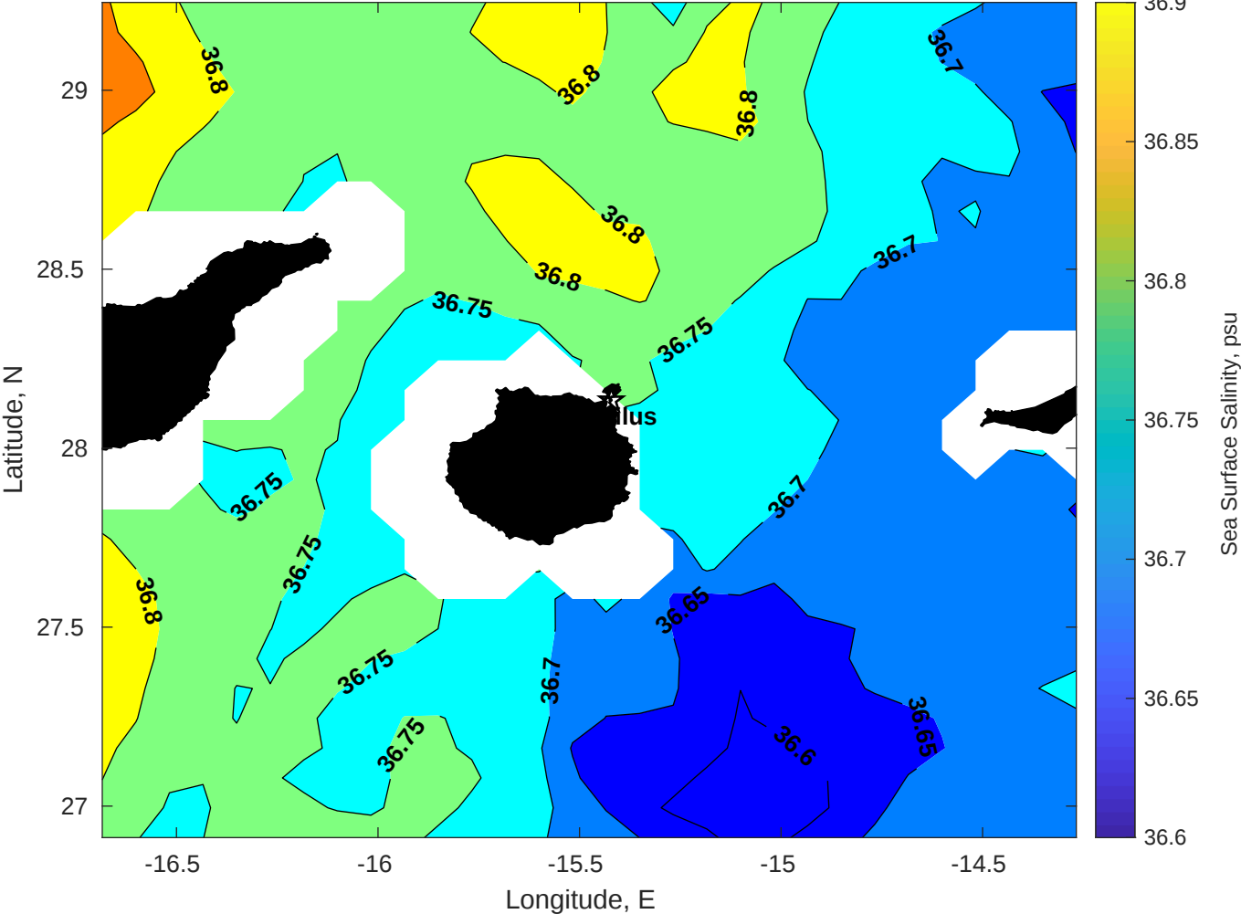
Surface Salinity for Nautilus at 27-Jan-2026 00:00:00
