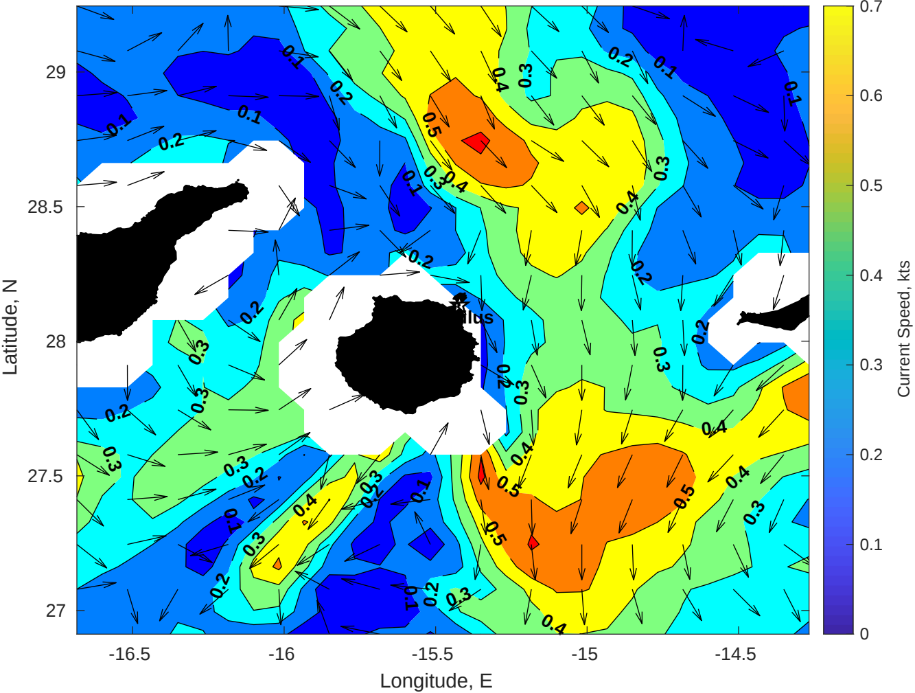
Surface Currents for Nautilus at 27-Jan-2026 00:00:00
