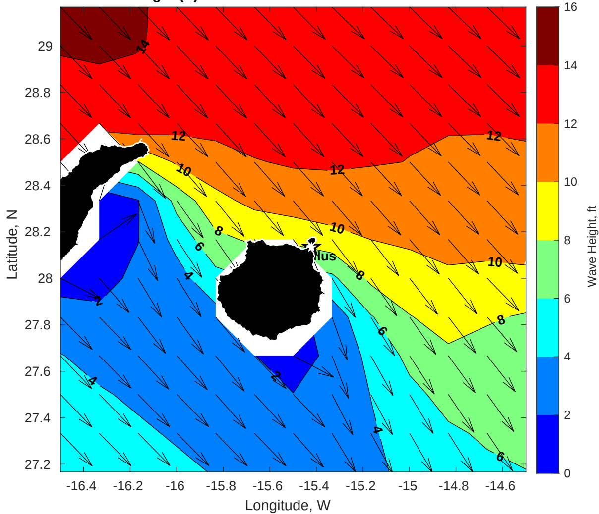
GFS Wave Height (ft) for Nautilus at 28-Jan-2026 09:00:00
