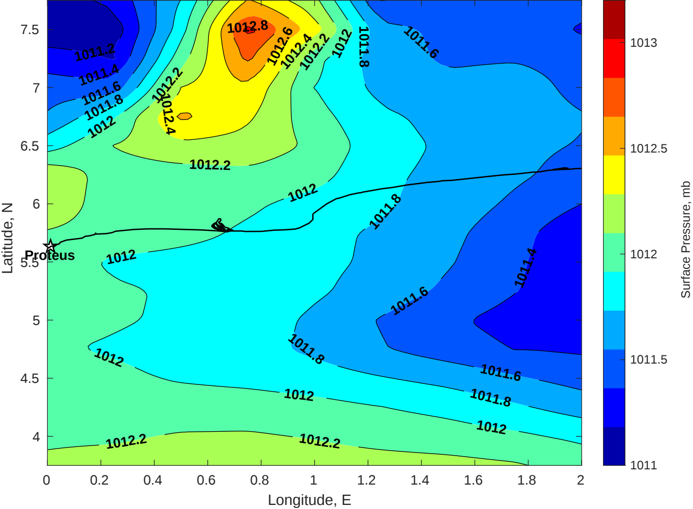
Surface Pressure (mb) for Proteus at 29-Jan-2026 00:00:00
