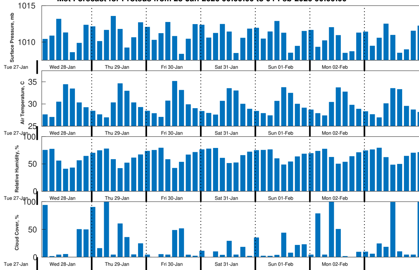
Met Forecast for Proteus from 28-Jan-2026 00:00:00 to 04-Feb-2026 00:00:00
