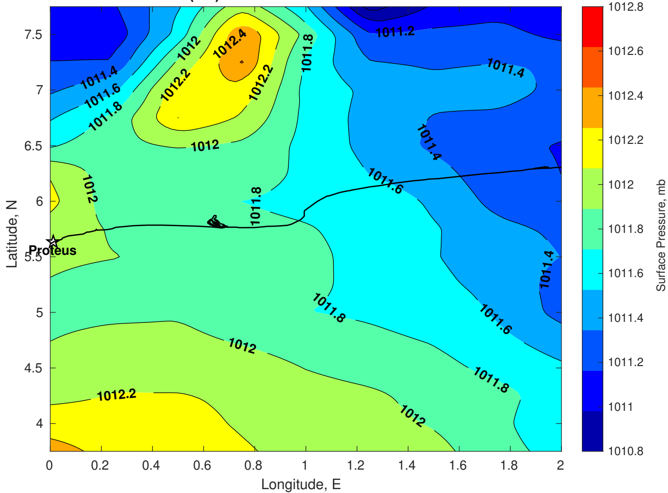
Surface Pressure (mb) for Proteus at 30-Jan-2026 00:00:00
