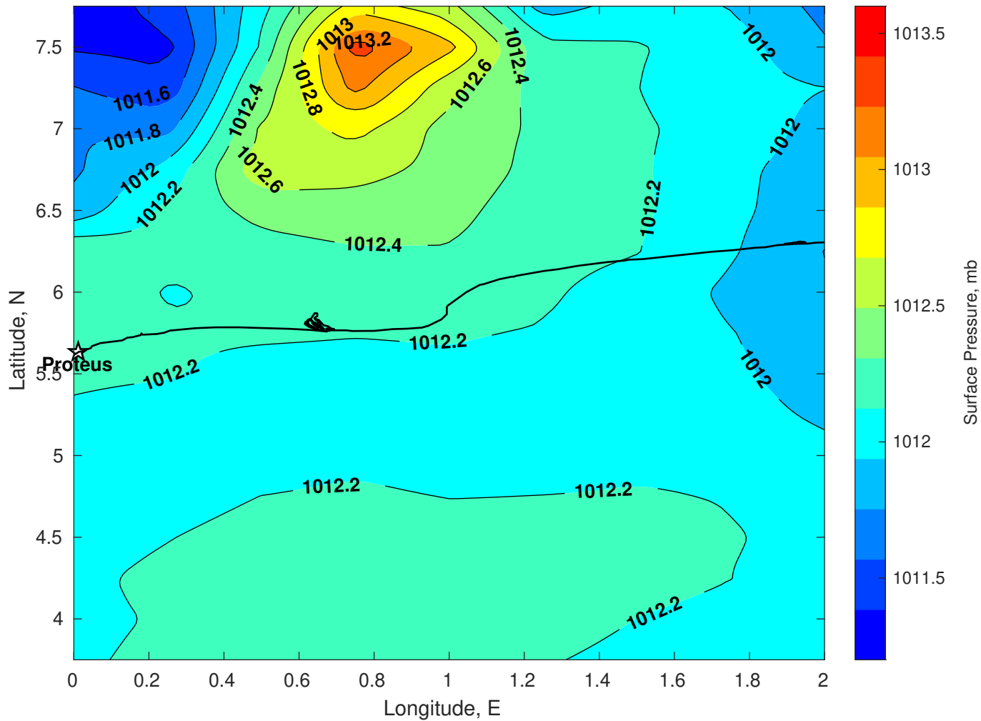
Surface Pressure (mb) for Proteus at 28-Jan-2026 00:00:00
