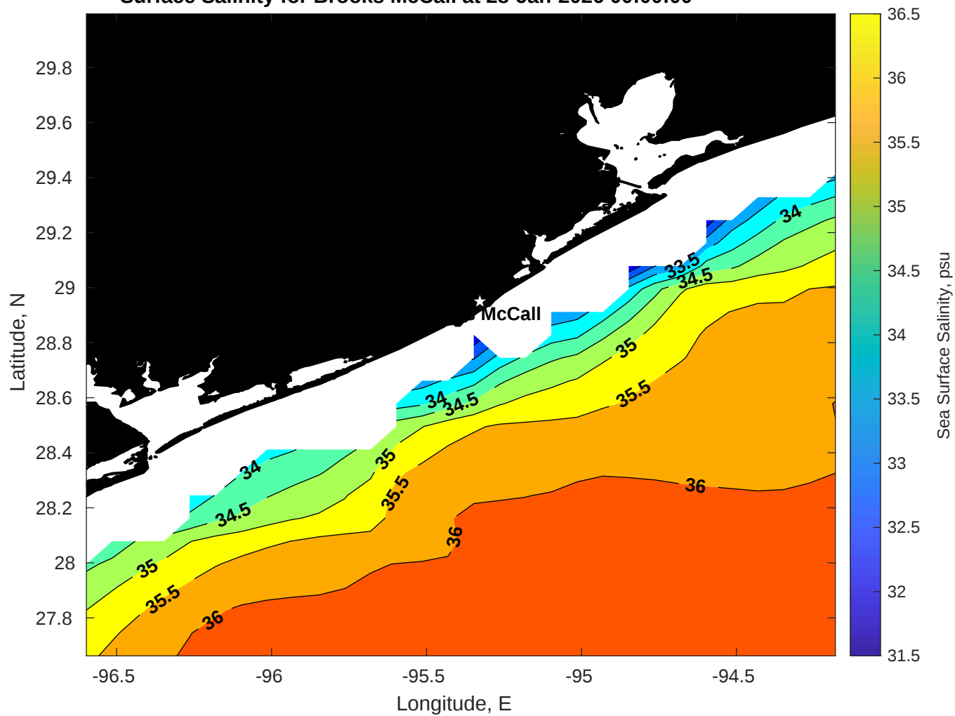
Surface Salinity for Brooks McCall at 28-Jan-2026 00:00:00
