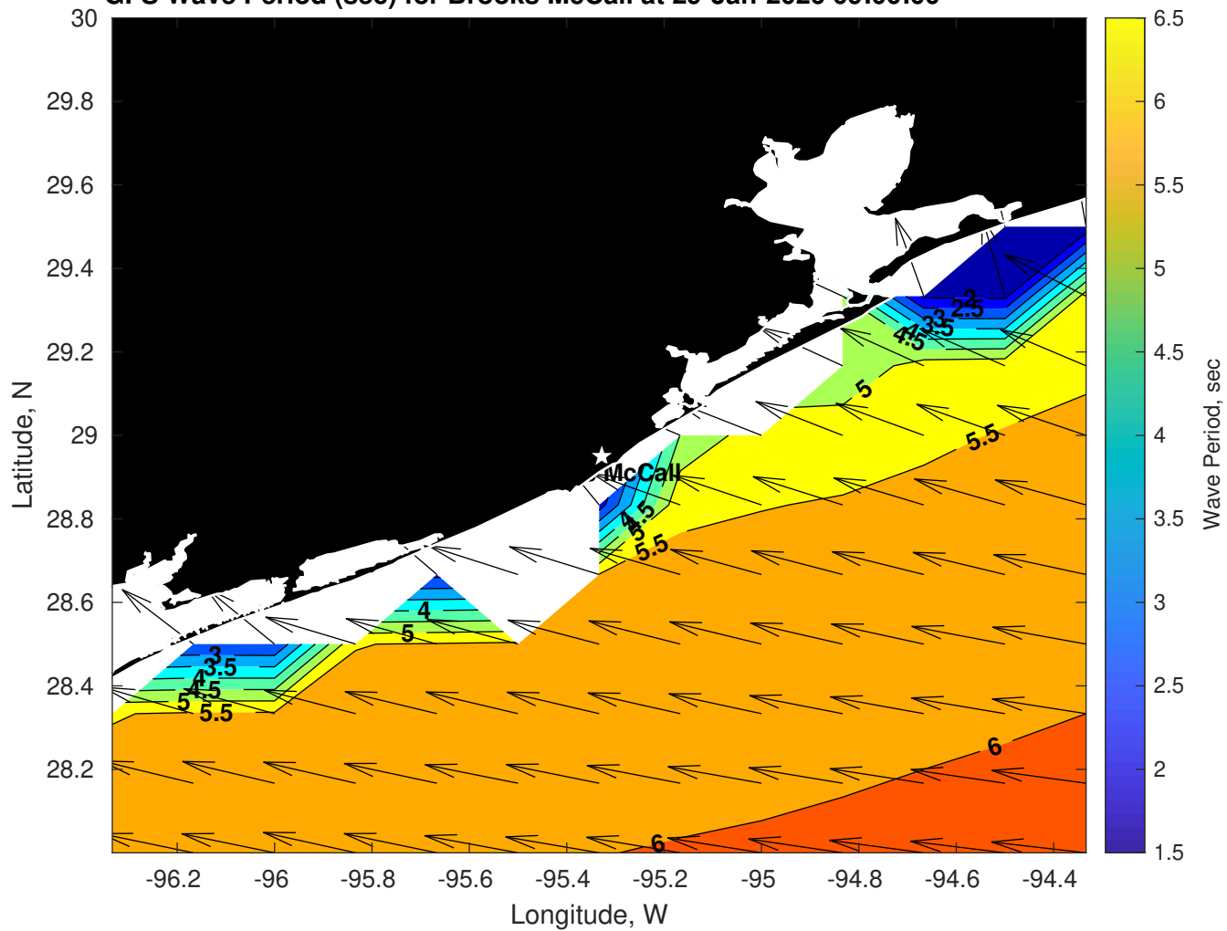
GFS Wave Period (sec) for Brooks McCall at 29-Jan-2026 09:00:00
