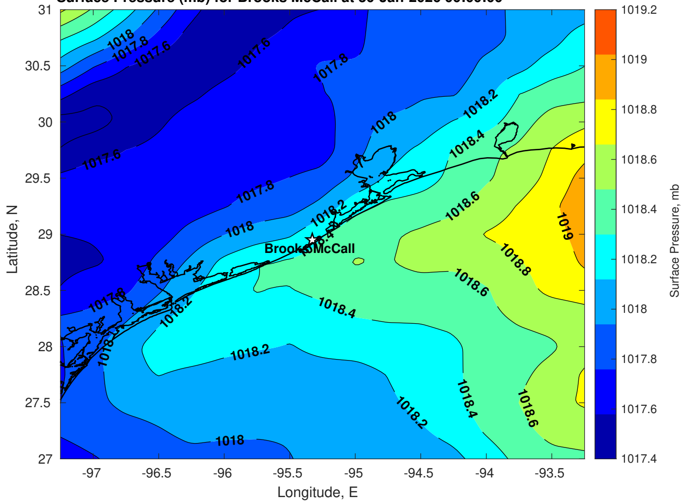
Surface Pressure (mb) for Brooks McCall at 30-Jan-2026 00:00:00
