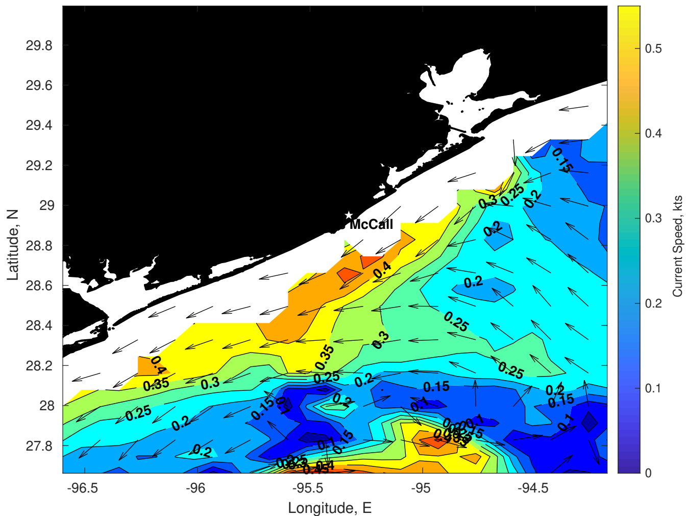
Surface Currents for Brooks McCall at 28-Jan-2026 00:00:00
