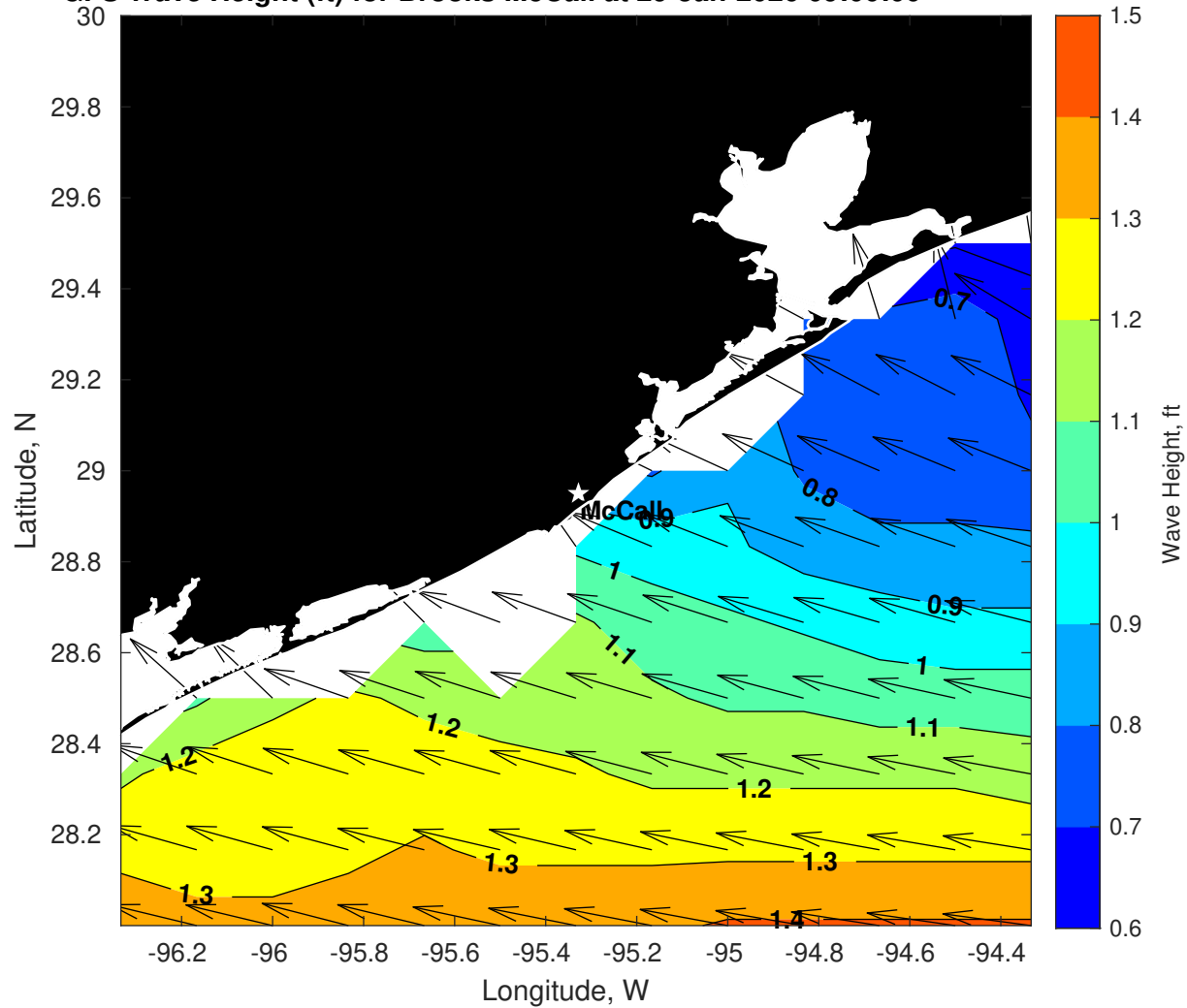
GFS Wave Height (ft) for Brooks McCall at 29-Jan-2026 09:00:00
