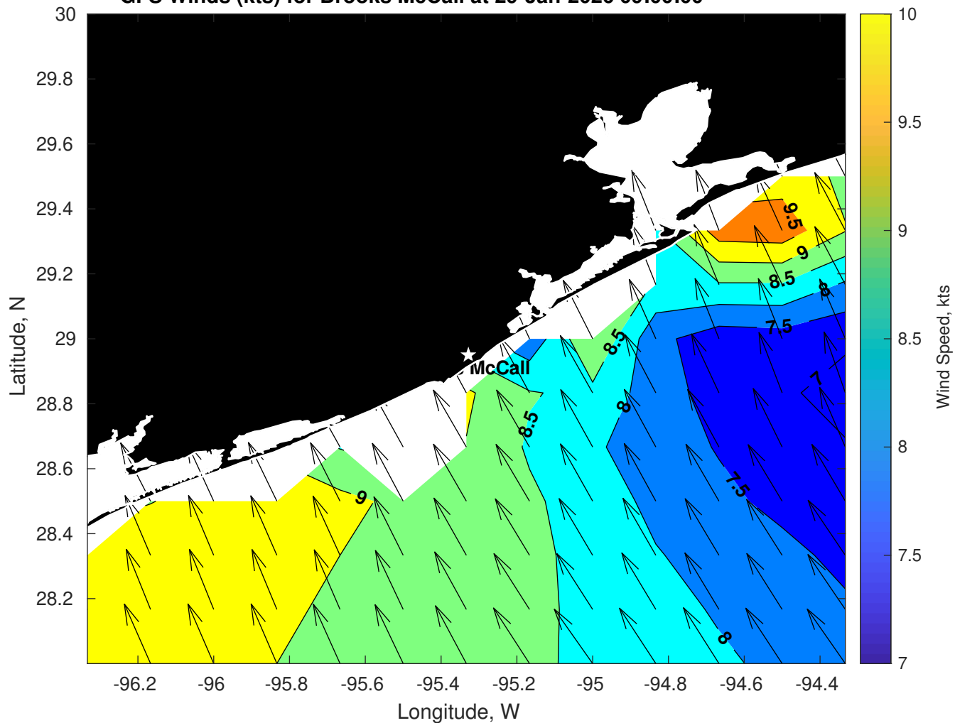
GFS Winds (kts) for Brooks McCall at 29-Jan-2026 09:00:00
