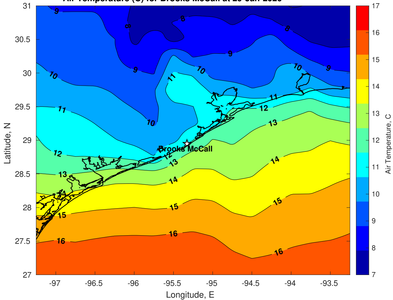
Air Temperature (C) for Brooks McCall at 29-Jan-2026
