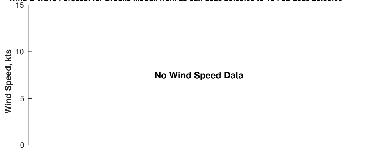
Wind & Wave Forecast for Brooks McCall from 28-Jan-2026 20:00:00 to 13-Feb-2026 20:00:00
