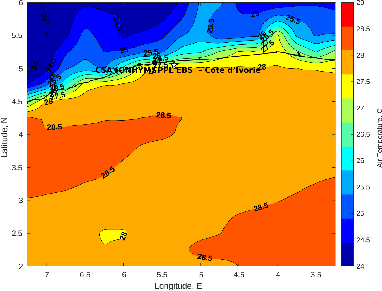
Air Temperature (C) for CSA (ONHYM) PPL EBS - Cote d'Ivoire at 29-Jan-2026
