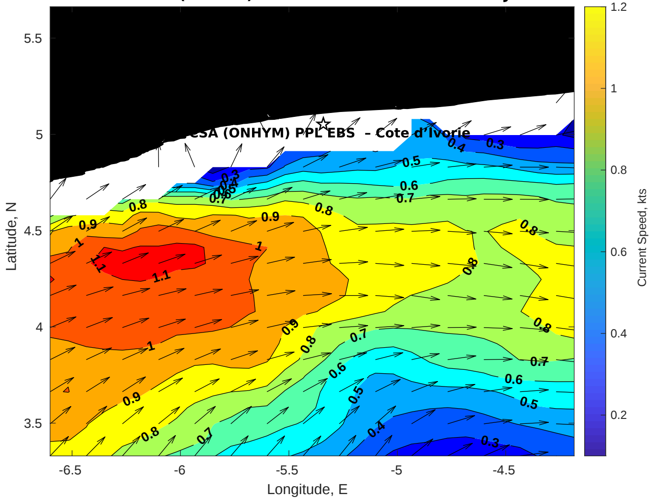
Surface Currents for CSA (ONHYM) PPL EBS - Cote d'Ivoire at 28-Jan-2026 00:00:00
