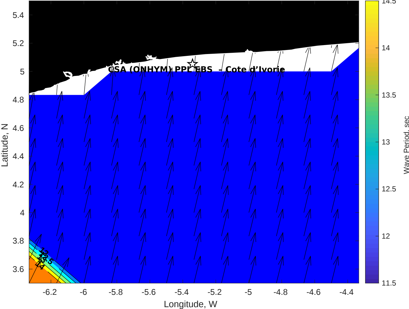
GFS Wave Period (sec) for CSA (ONHYM) PPL EBS - Cote d'Ivoire at 29-Jan-2026 09:00:00
