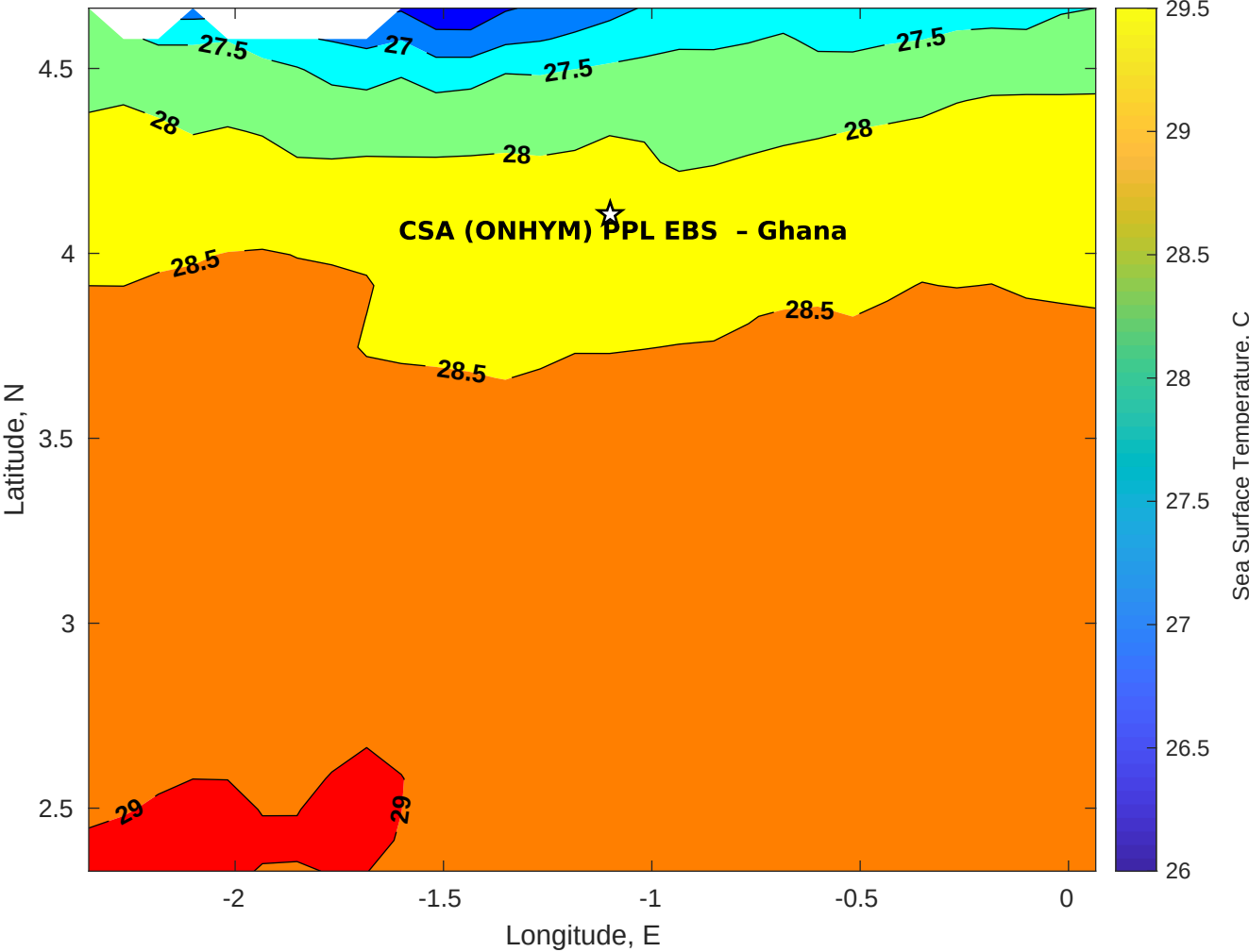
SST for CSA (ONHYM) PPL EBS - Ghana at 28-Jan-2026 00:00:00
