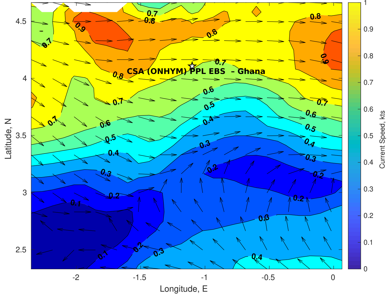
Surface Currents for CSA (ONHYM) PPL EBS - Ghana at 28-Jan-2026 00:00:00
