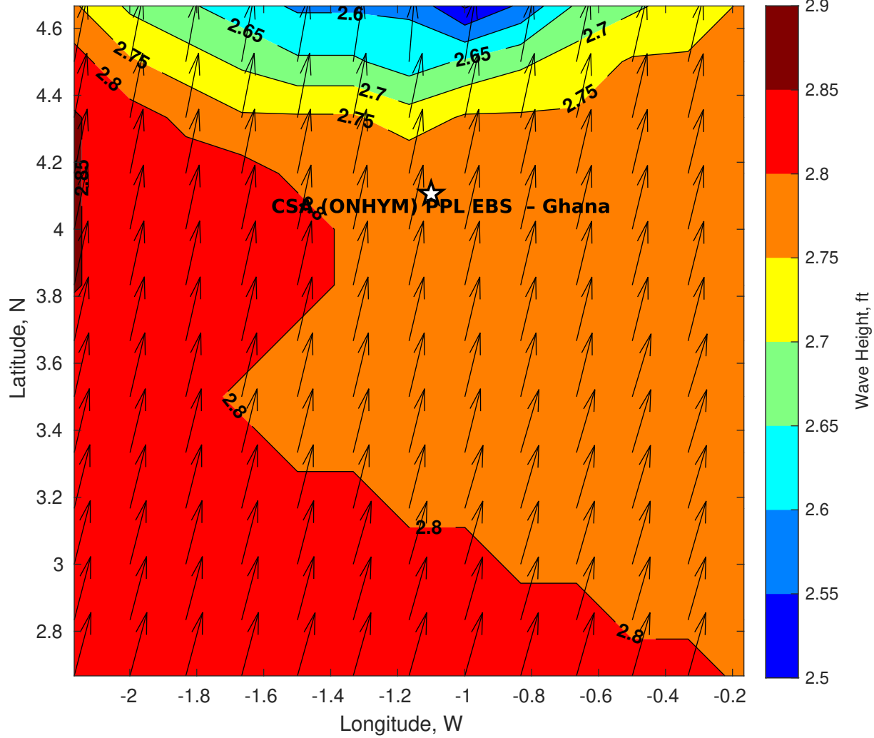
GFS Wave Height (ft) for CSA (ONHYM) PPL EBS - Ghana at 29-Jan-2026 09:00:00
