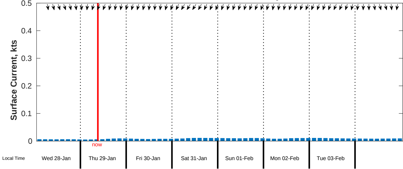
Surface Current Forecast for CSA (ONHYM) PPL EBS - Ghana from 28-Jan-2026 00:00:00 to 05-Feb-2026 00:00:00
