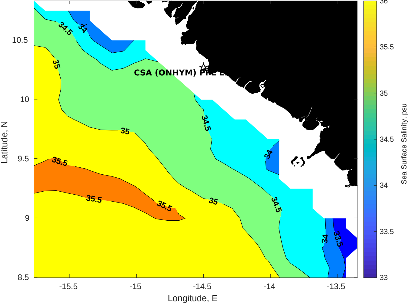
Surface Salinity for CSA (ONHYM) PPL EBS - Guinea at 28-Jan-2026 00:00:00
