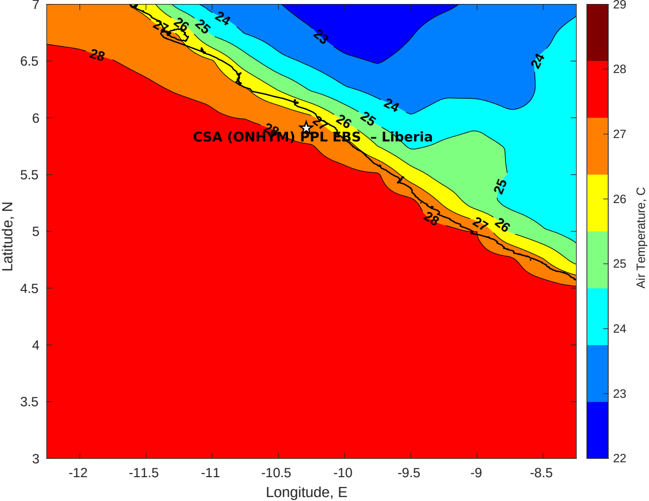
Air Temperature (C) for CSA (ONHYM) PPL EBS - Liberia at 29-Jan-2026
