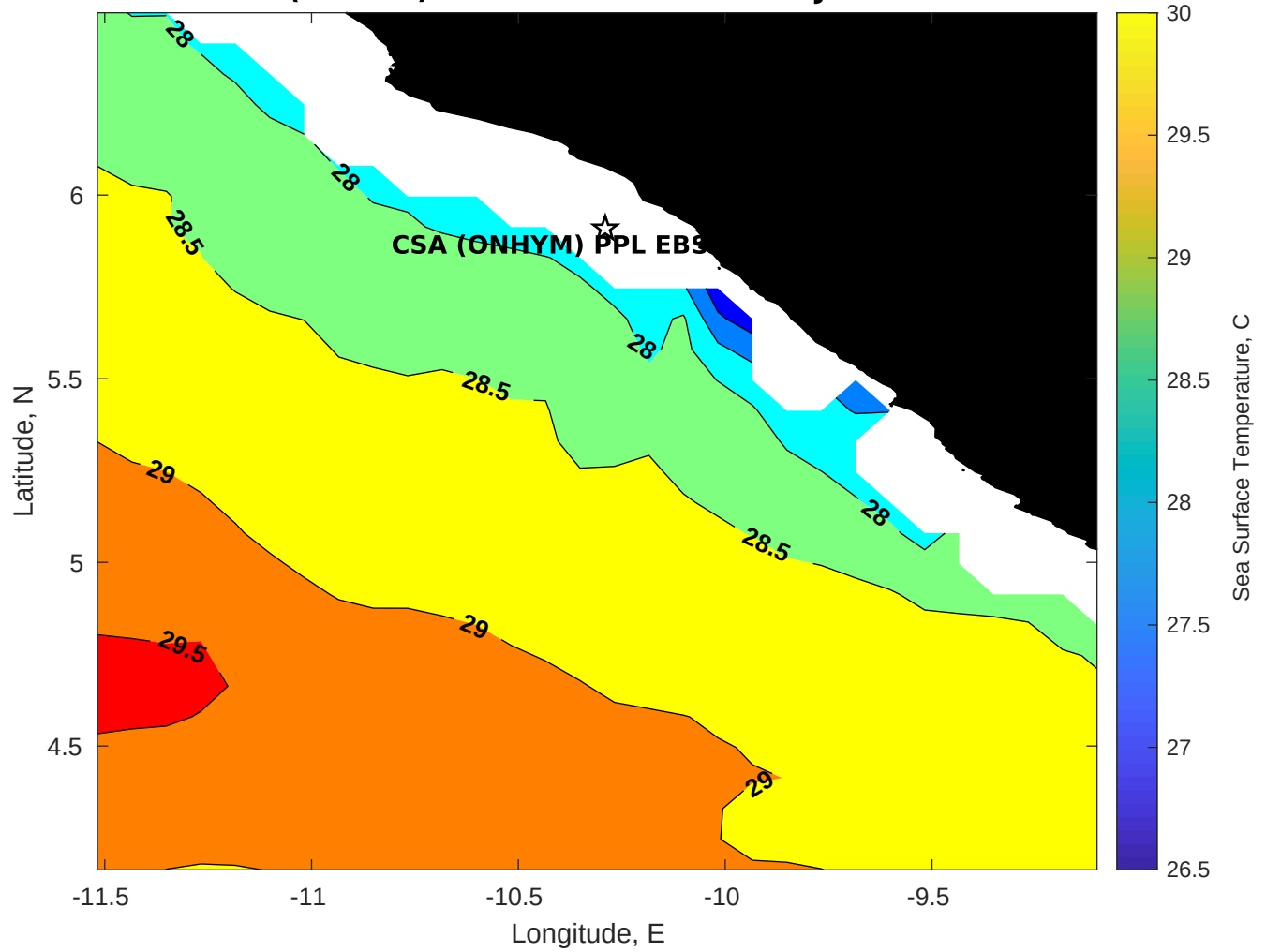
SST for CSA (ONHYM) PPL EBS - Liberia at 28-Jan-2026 00:00:00
