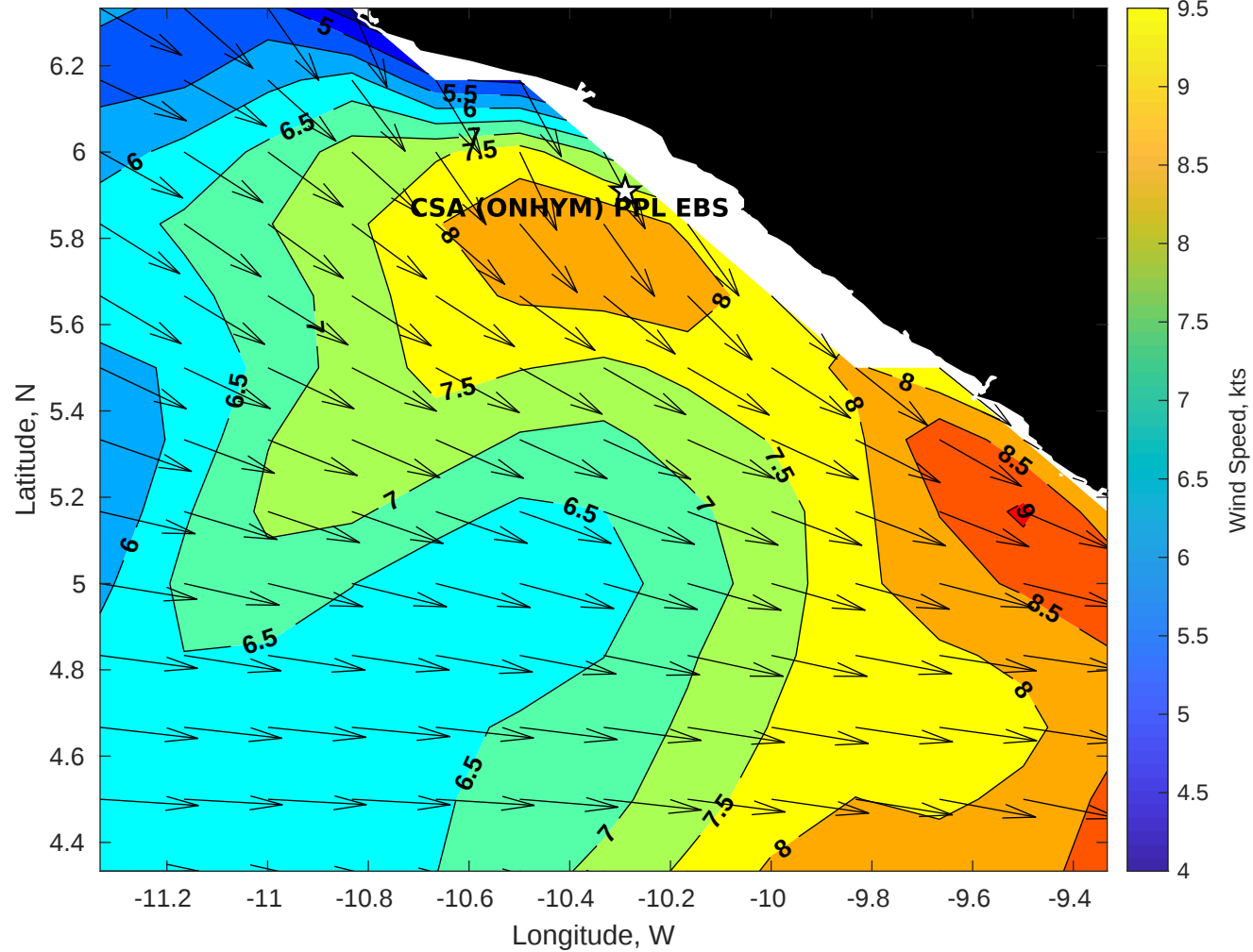
GFS Winds (kts) for CSA (ONHYM) PPL EBS - Liberia at 29-Jan-2026 09:00:00
