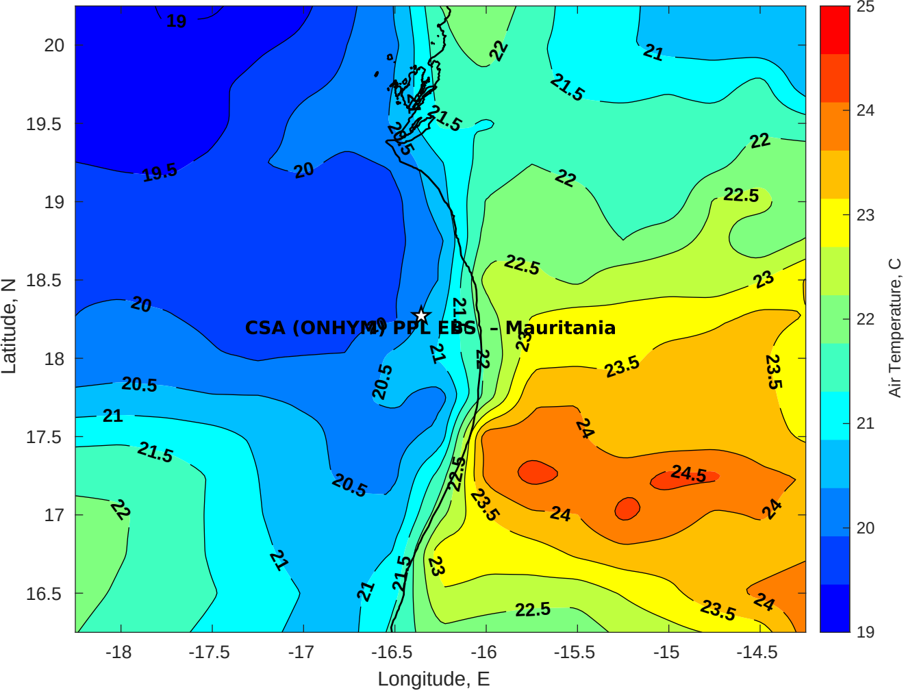
Air Temperature (C) for CSA (ONHYM) PPL EBS - Mauritania at 29-Jan-2026
