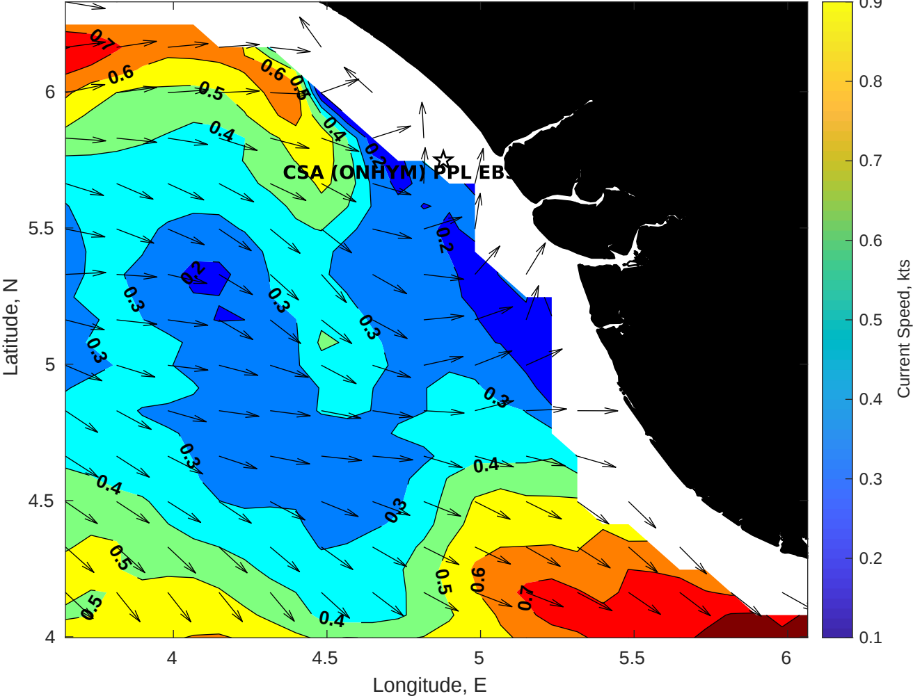
Surface Currents for CSA (ONHYM) PPL EBS - Nigeria at 28-Jan-2026 00:00:00
