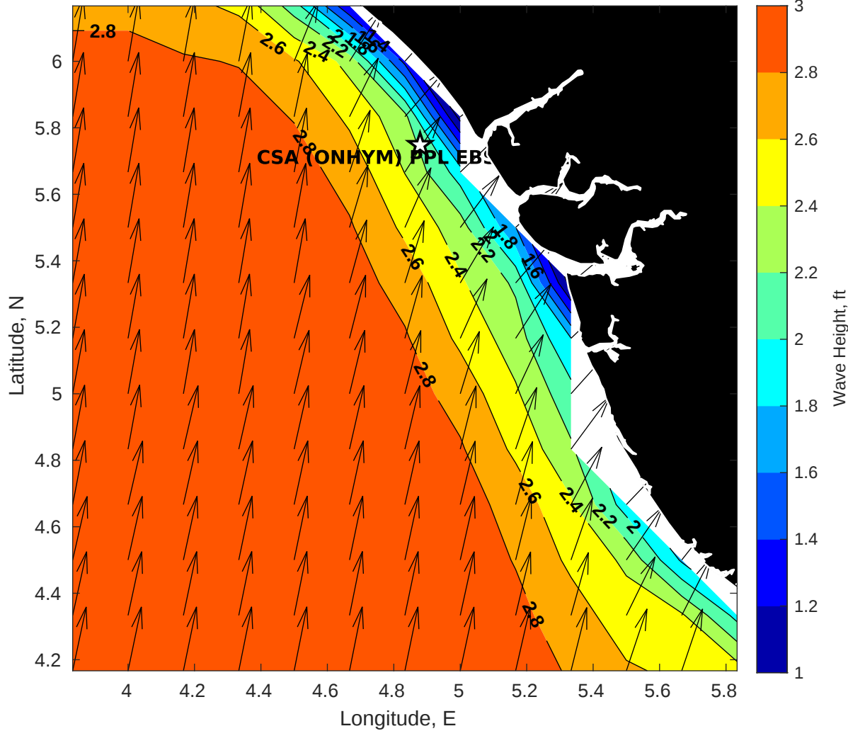
GFS Wave Height (ft) for CSA (ONHYM) PPL EBS - Nigeria at 29-Jan-2026 09:00:00
