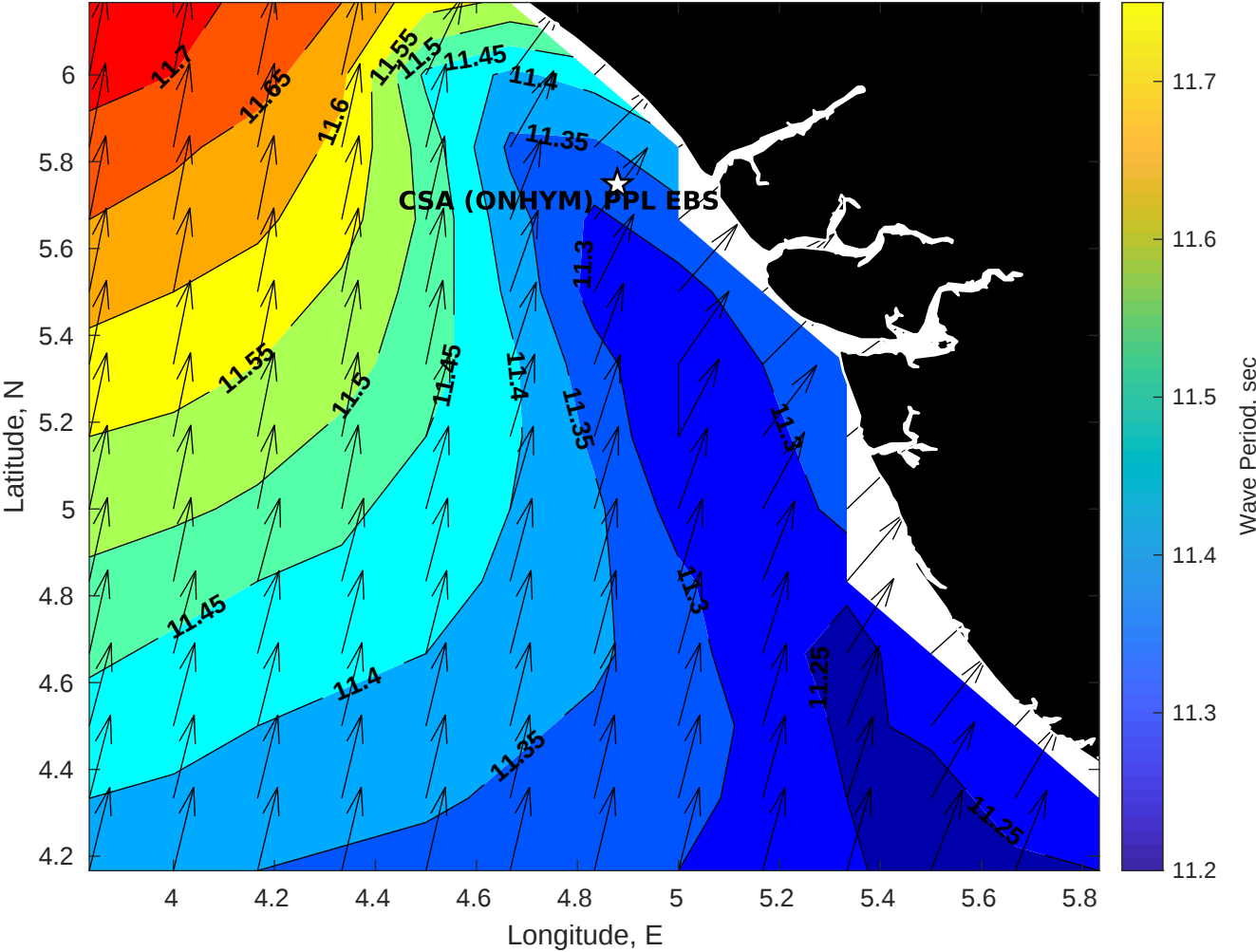
GFS Wave Period (sec) for CSA (ONHYM) PPL EBS - Nigeria at 29-Jan-2026 09:00:00
