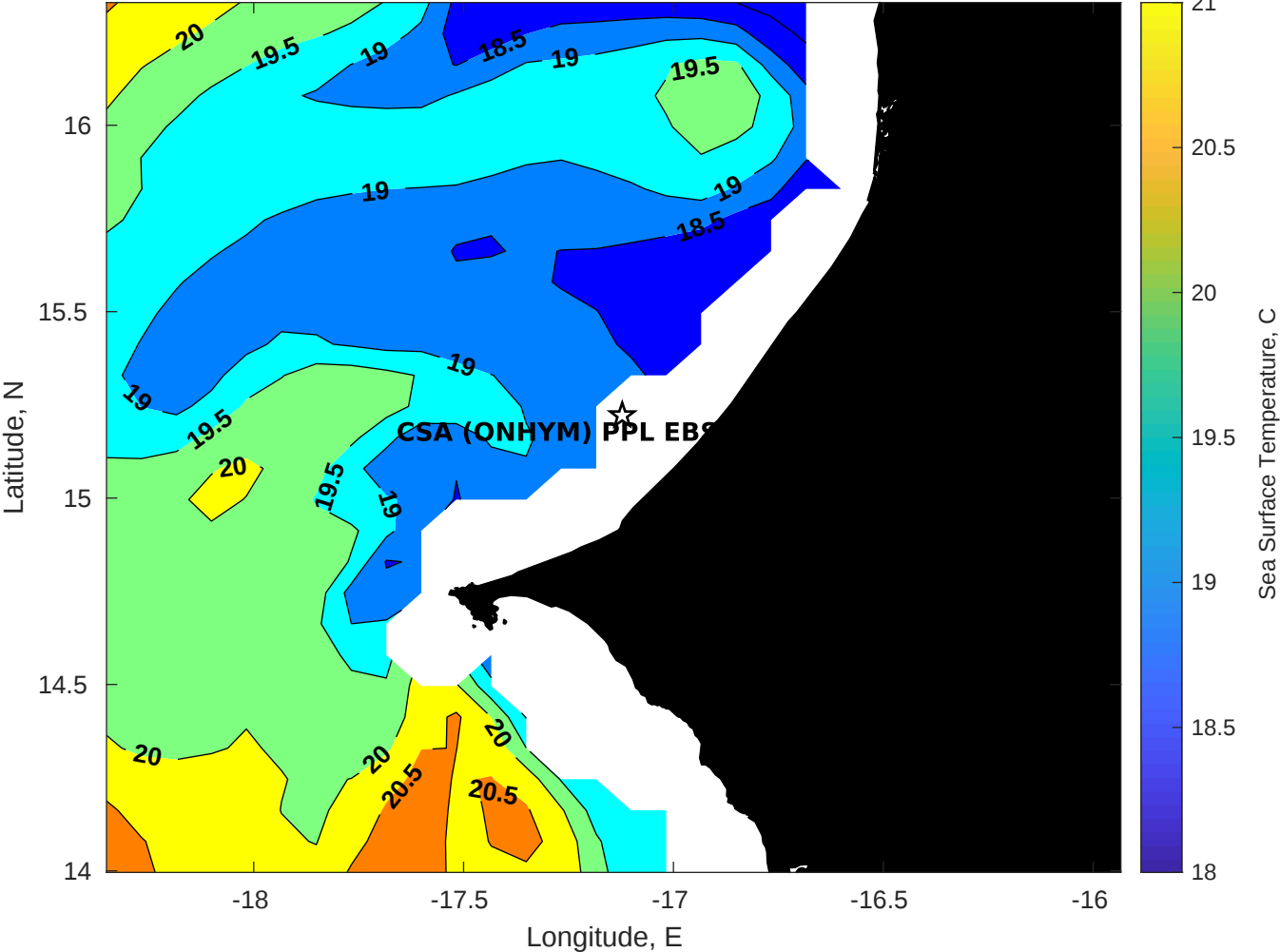
SST for CSA (ONHYM) PPL EBS - Senegal at 28-Jan-2026 00:00:00
