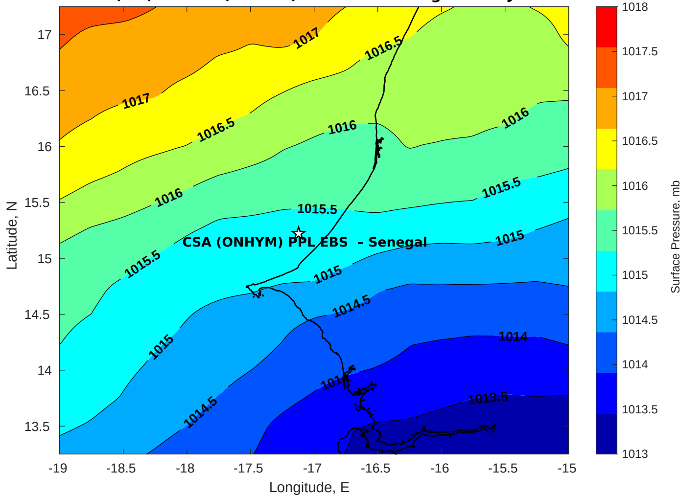
Surface Pressure (mb) for CSA (ONHYM) PPL EBS - Senegal at 29-Jan-2026 00:00:00
