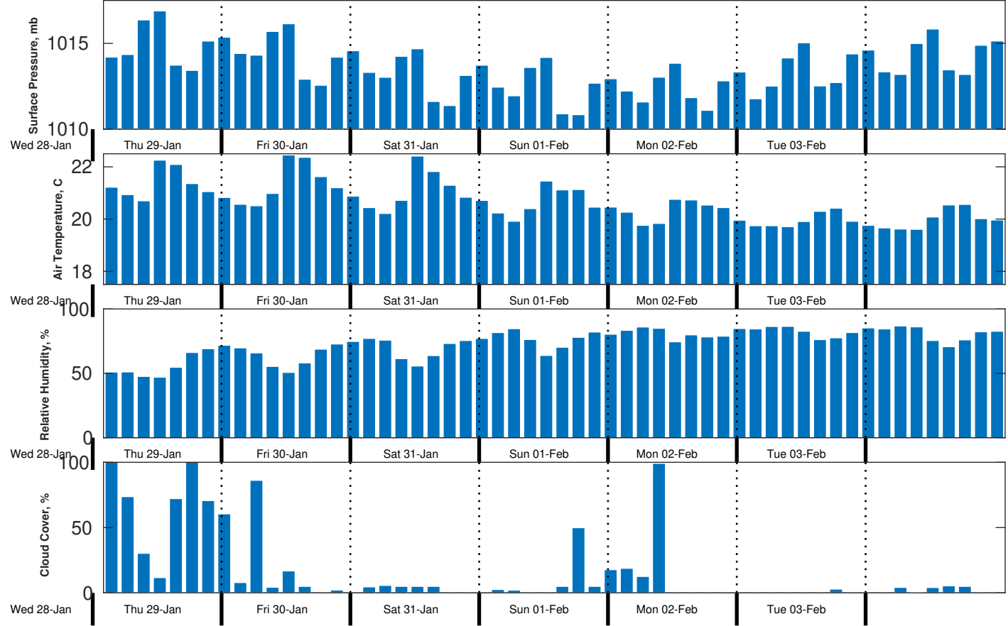
Met Forecast for CSA (ONHYM) PPL EBS - Senegal from 29-Jan-2026 00:00:00 to 05-Feb-2026 00:00:00
