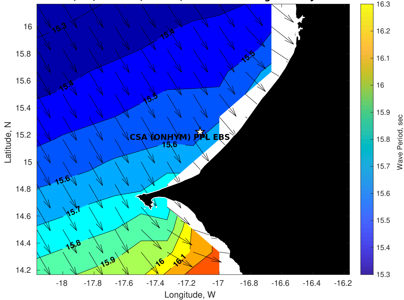
GFS Wave Period (sec) for CSA (ONHYM) PPL EBS - Senegal at 29-Jan-2026 09:00:00
