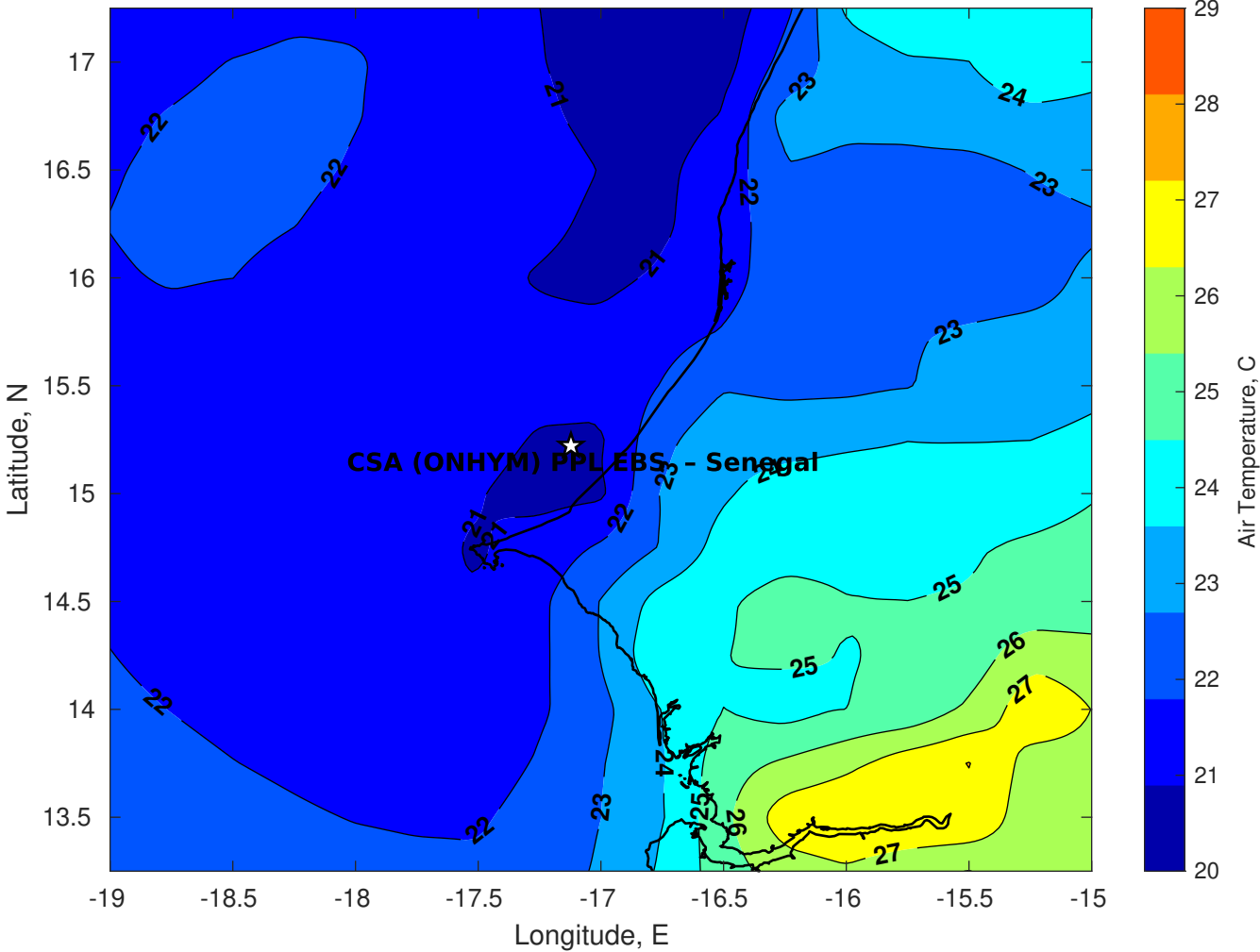
Air Temperature (C) for CSA (ONHYM) PPL EBS - Senegal at 29-Jan-2026
