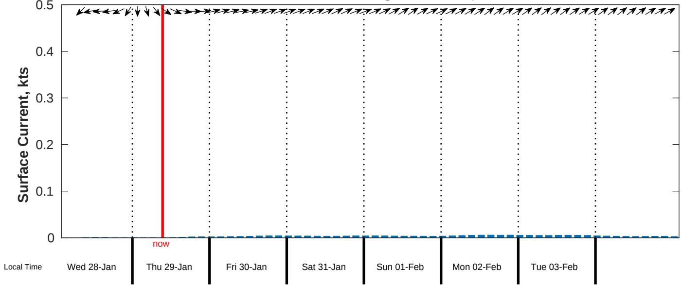
Surface Current Forecast for CSA (ONHYM) PPL EBS - Senegal from 28-Jan-2026 00:00:00 to 05-Feb-2026 00:00:00
