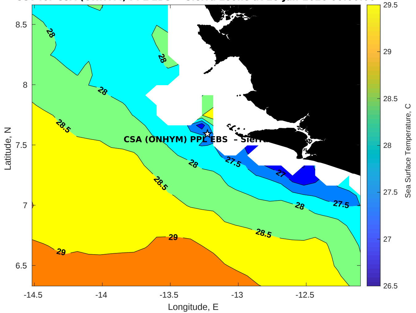
SST for CSA (ONHYM) PPL EBS - Sierra Leone at 28-Jan-2026 00:00:00
