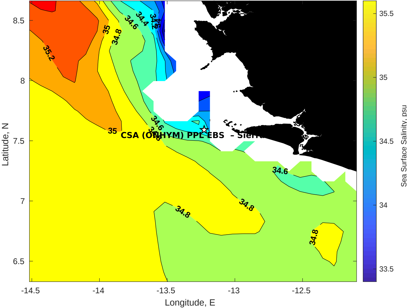
Surface Salinity for CSA (ONHYM) PPL EBS - Sierra Leone at 28-Jan-2026 00:00:00
