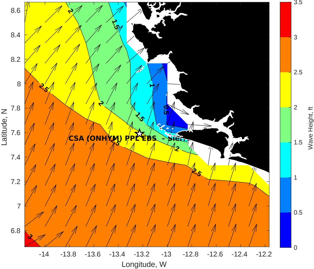
GFS Wave Height (ft) for CSA (ONHYM) PPL EBS - Sierra Leone at 29-Jan-2026 09:00:00
