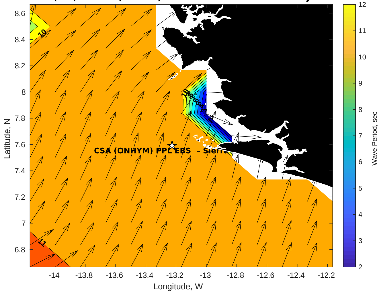
GFS Wave Period (sec) for CSA (ONHYM) PPL EBS - Sierra Leone at 29-Jan-2026 09:00:00
